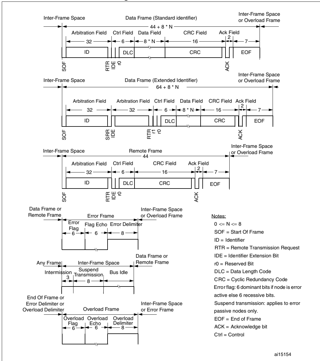
Figure 310. CAN frames
