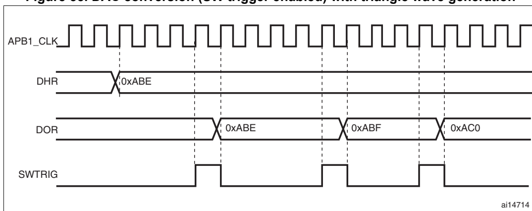
Figure 55. DAC conversion (SW trigger enabled) with triangle wave generation
