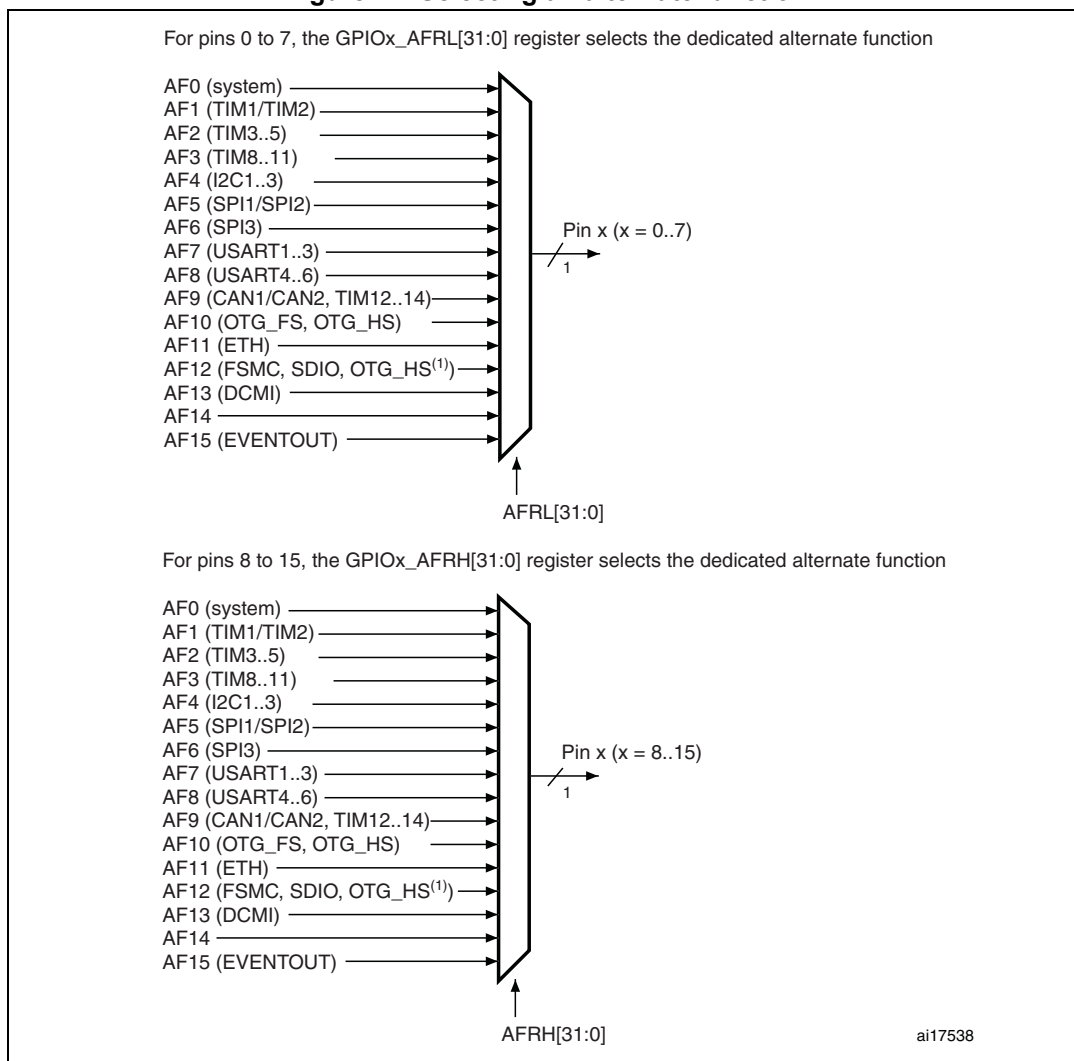
Figure 14. Selecting an alternate function
