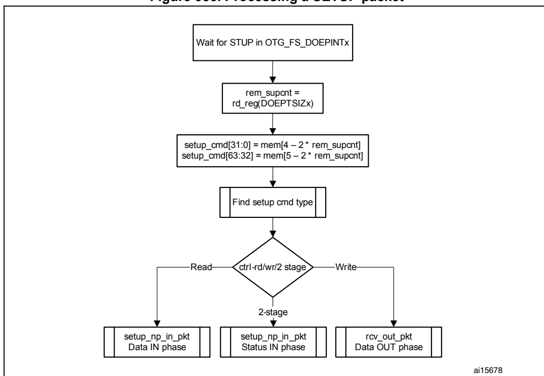
Figure 388. Processing a SETUP packet
