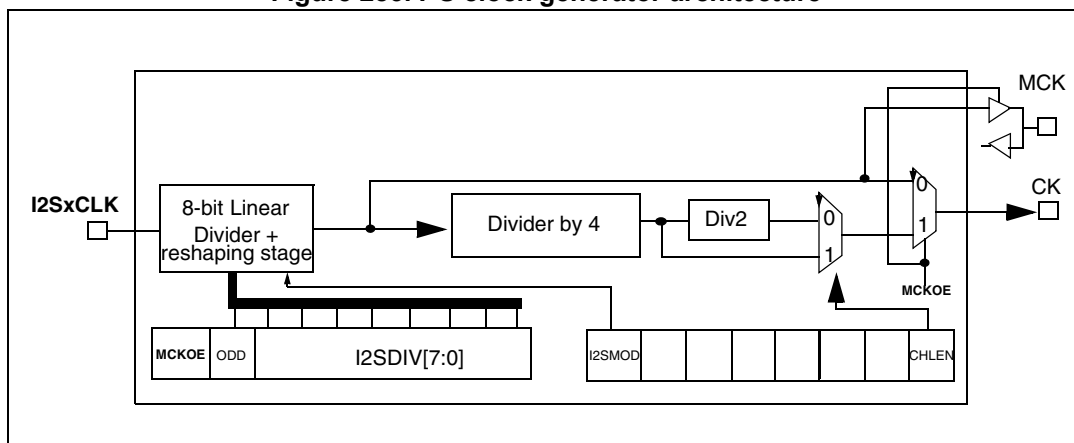
Figure 283. I 2 S clock generator architecture
