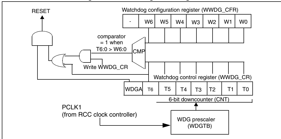
Figure 193. Watchdog block diagram
