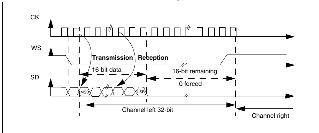
Figure 269. I 2 S Philips standard (16-bit extended to 32-bit packet frame with CPOL = 0)
