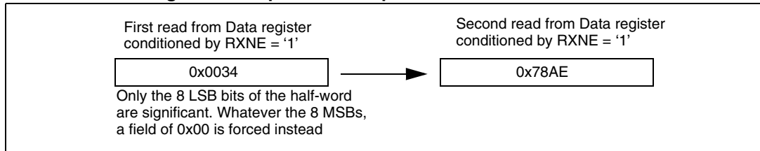
Figure 277. Operations required to receive 0x3478AE
