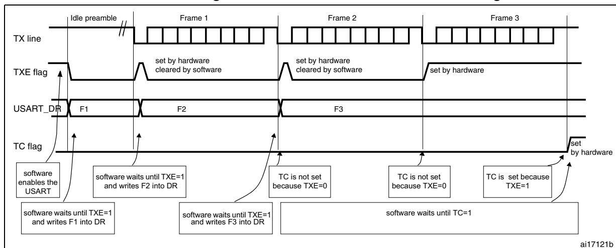
Figure 226. TC/TXE behavior when transmitting
