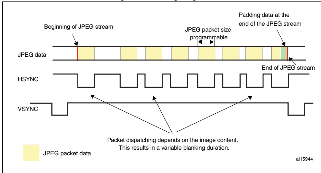
Figure 59. Timing diagram
