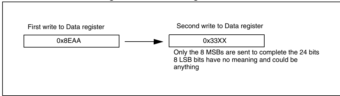
Figure 267. Transmitting 0x8EAA33
