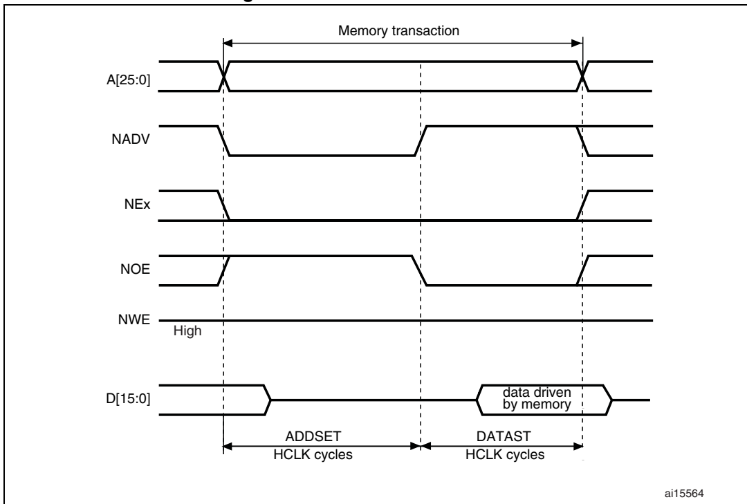
Figure 404. Mode C read accesses
