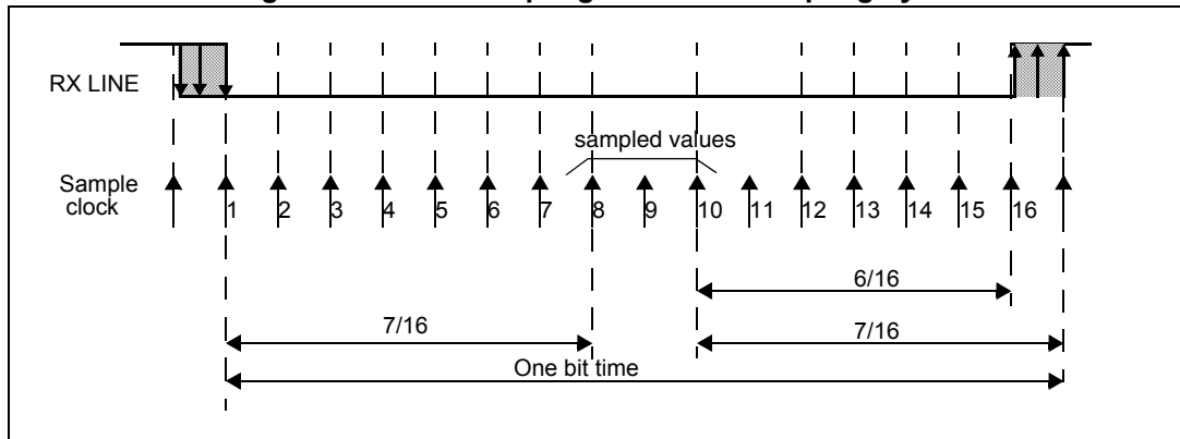
Figure 228. Data sampling when oversampling by 16
