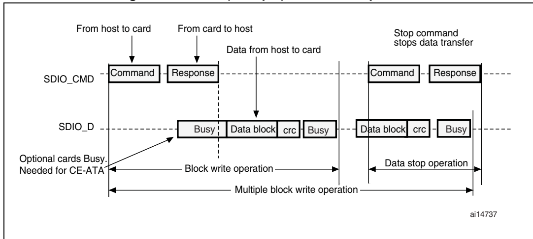
Figure 286. SDIO (multiple) block write operation
