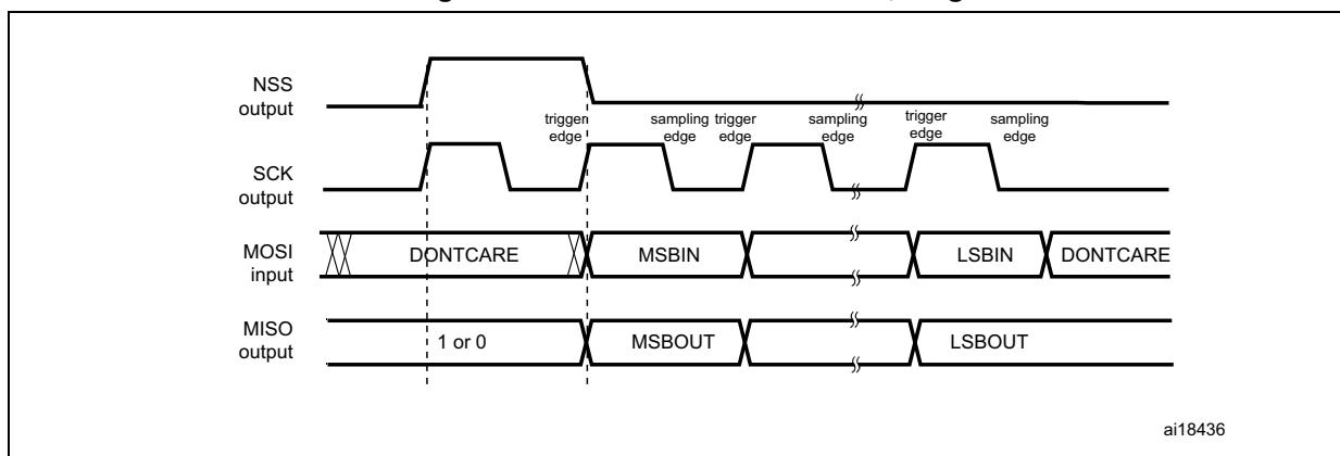
Figure 253. TI mode - master mode, single transfer
