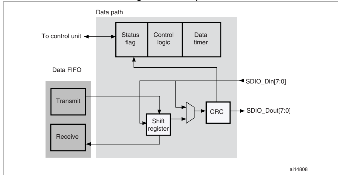
Figure 295. Data path
