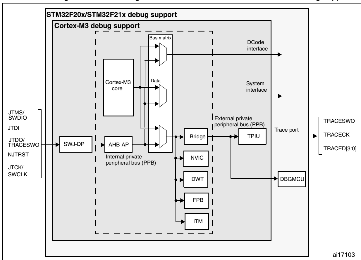
Figure 417. Block diagram of STM32 MCU and Cortex™-M3-level debug support
