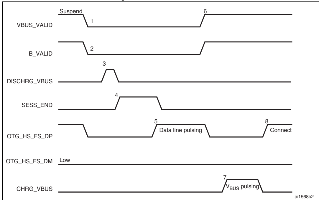
Figure 392. B-device SRP
