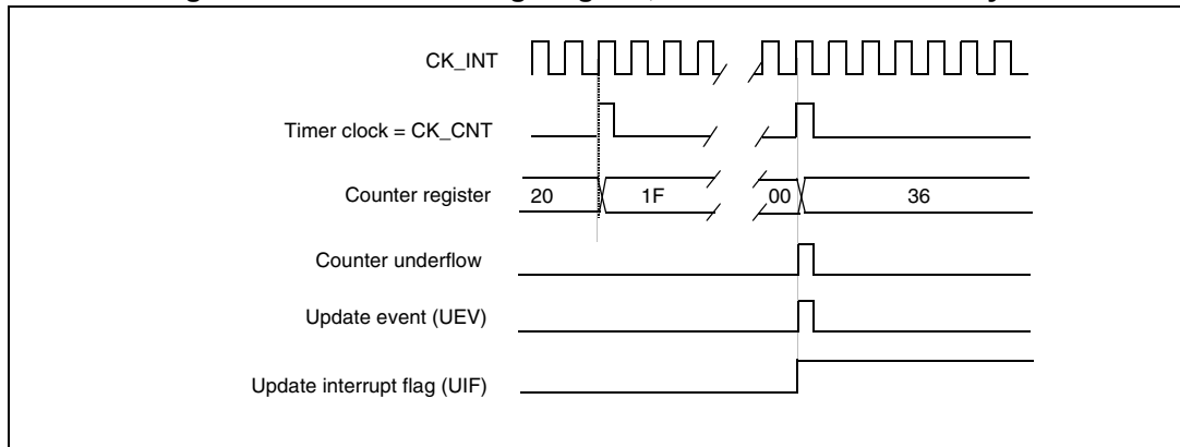
Figure 126. Counter timing diagram, Update event
