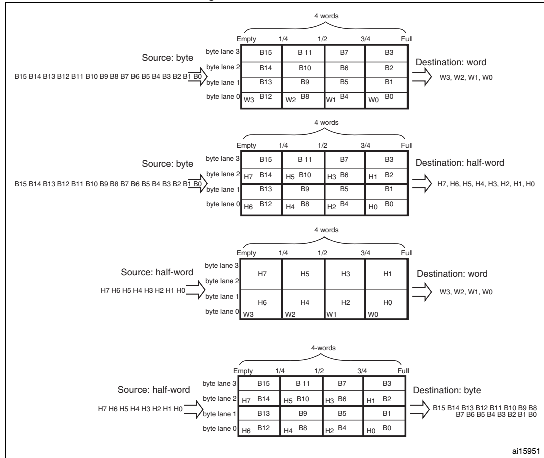
Figure 27. FIFO structure
