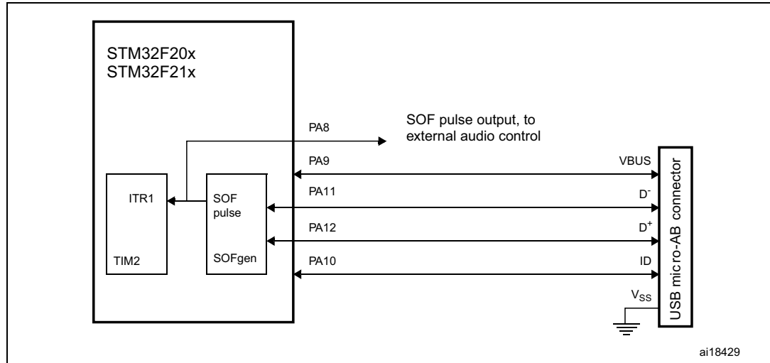
Figure 353. SOF connectivity
