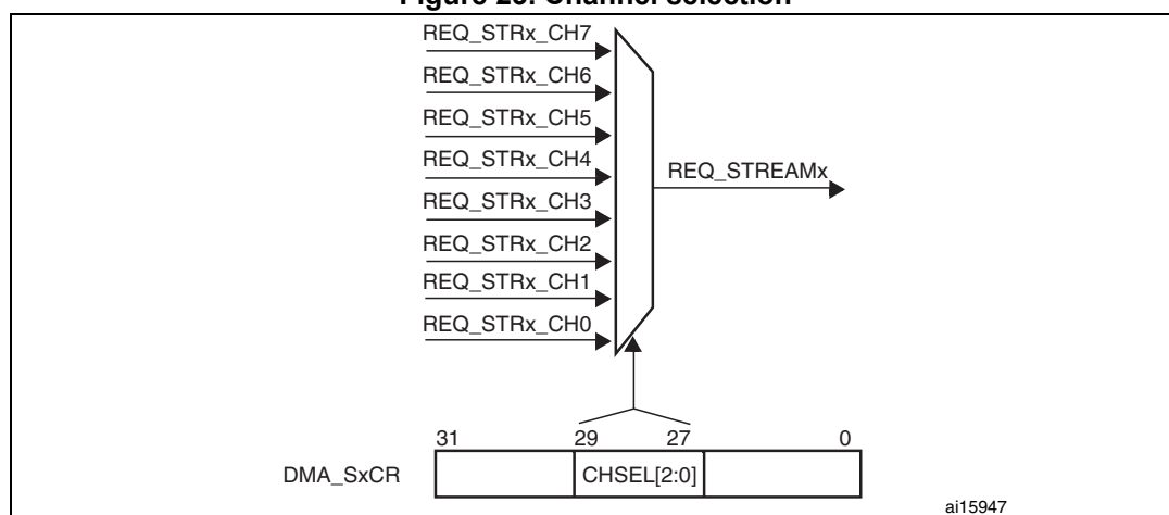
Figure 23. Channel selection
