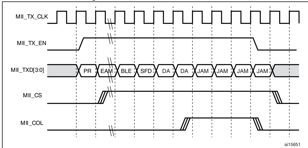
Figure 328 shows a frame transmission in MII and RMII.
