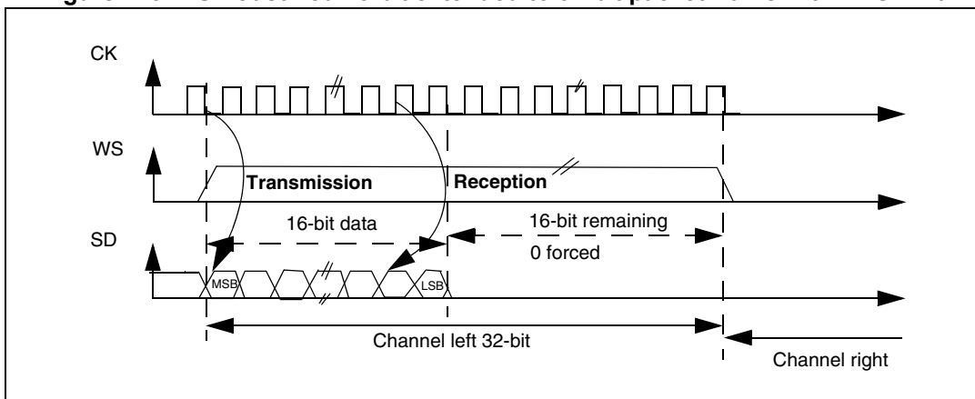
Figure 273. MSB Justified 16-bit extended to 32-bit packet frame with CPOL = 0
