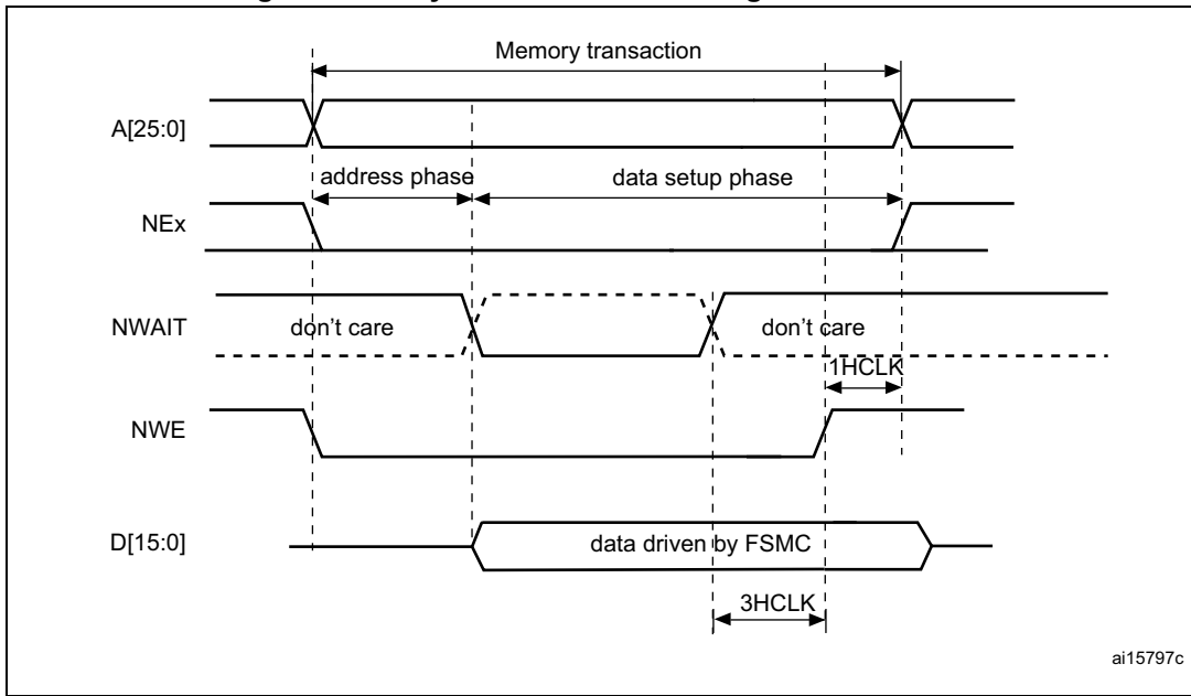
Figure 411. Asynchronous wait during a write access
