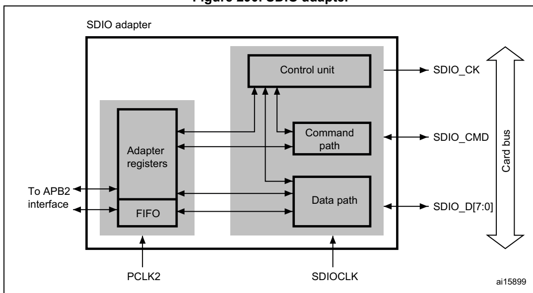
Figure 290. SDIO adapter
