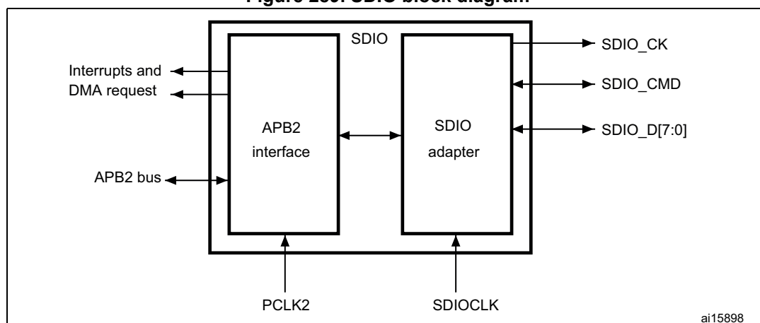
Figure 289. SDIO block diagram
