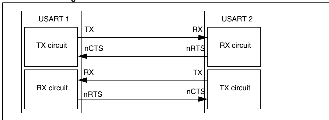
Figure 244. Hardware flow control between 2 USARTs
