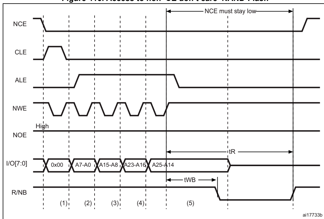
Figure 416. Access to non ‘CE don’t care’ NAND-Flash
