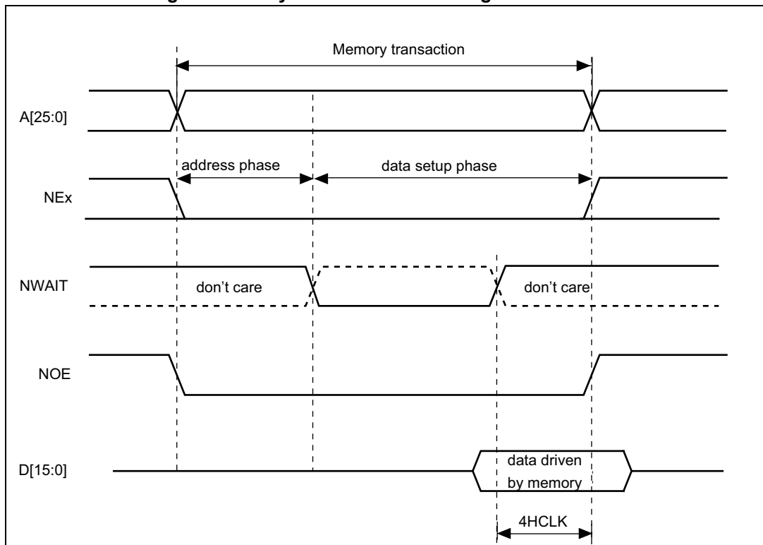
Figure 410. Asynchronous wait during a read access
