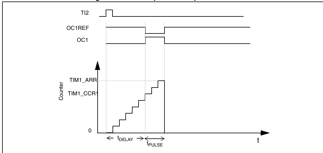
Figure 145. Example of one-pulse mode
