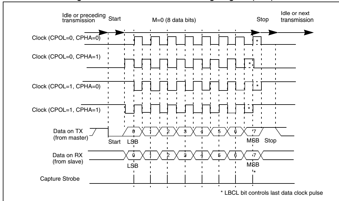
Figure 235. USART data clock timing diagram (M=0)
