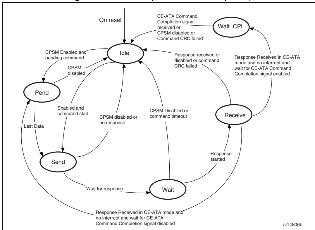
Figure 293. Command path state machine (CPSM)
