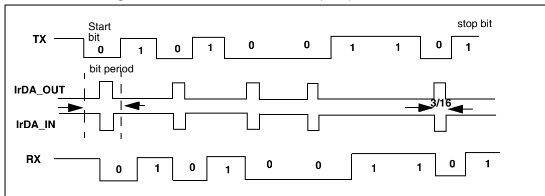
Figure 241. IrDA data modulation (3/16) -Normal mode
