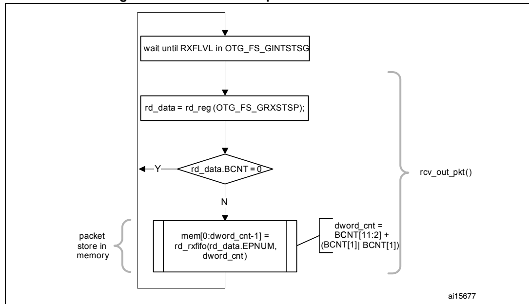
Figure 387. Receive FIFO packet read in slave mode
