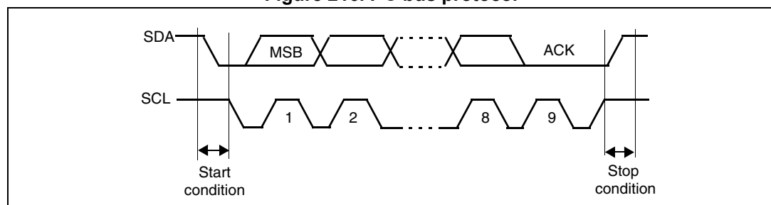
Figure 216. I 2 C bus protocol
