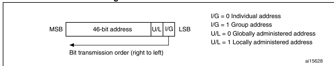
Figure 322. Address field format
