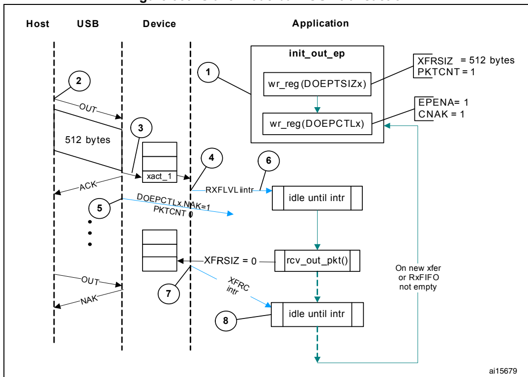
Figure 389. Slave mode bulk OUT transaction
