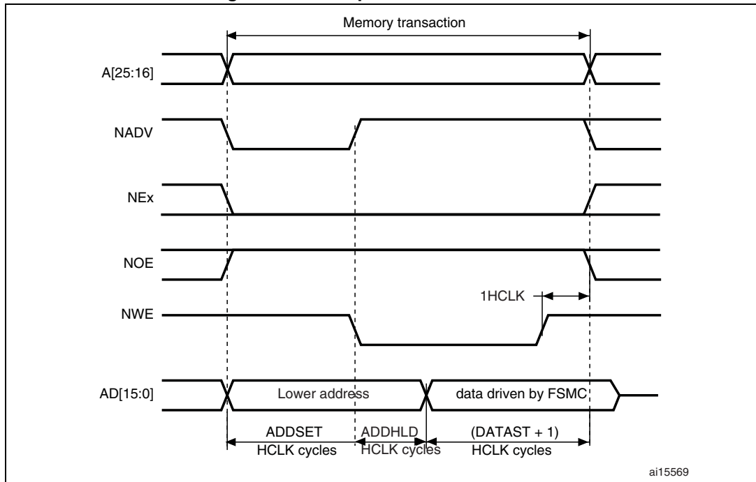
Figure 409. Multiplexed write accesses
