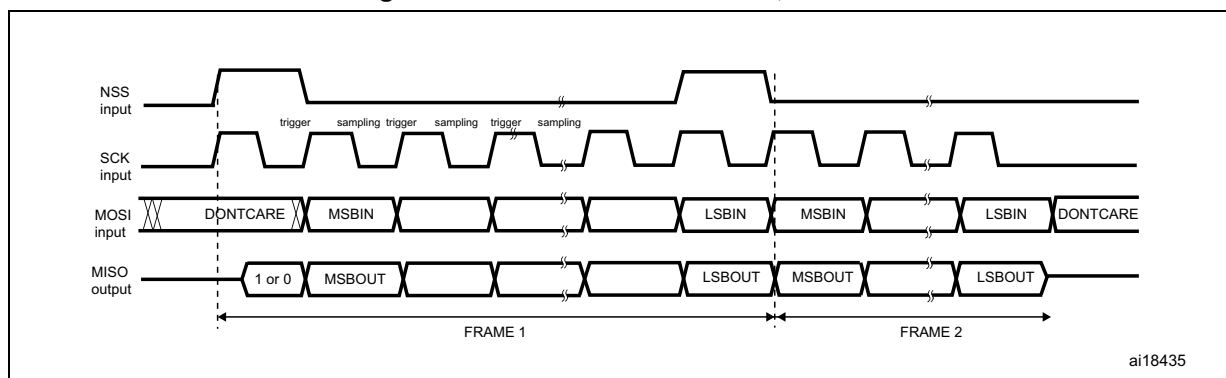
Figure 252. TI mode - Slave mode, continuous transfer
