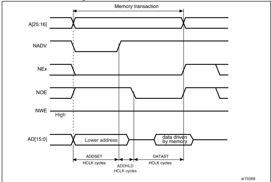
Figure 408. Multiplexed read accesses
