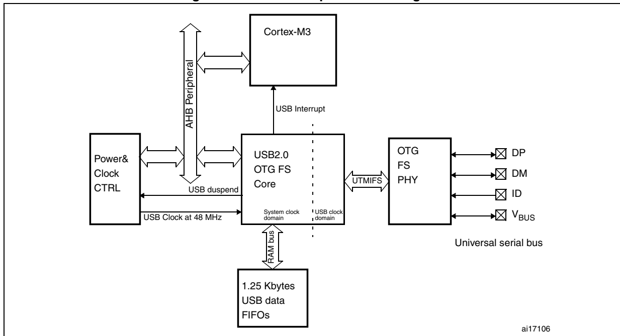
Figure 349. OTG full-speed block diagram
