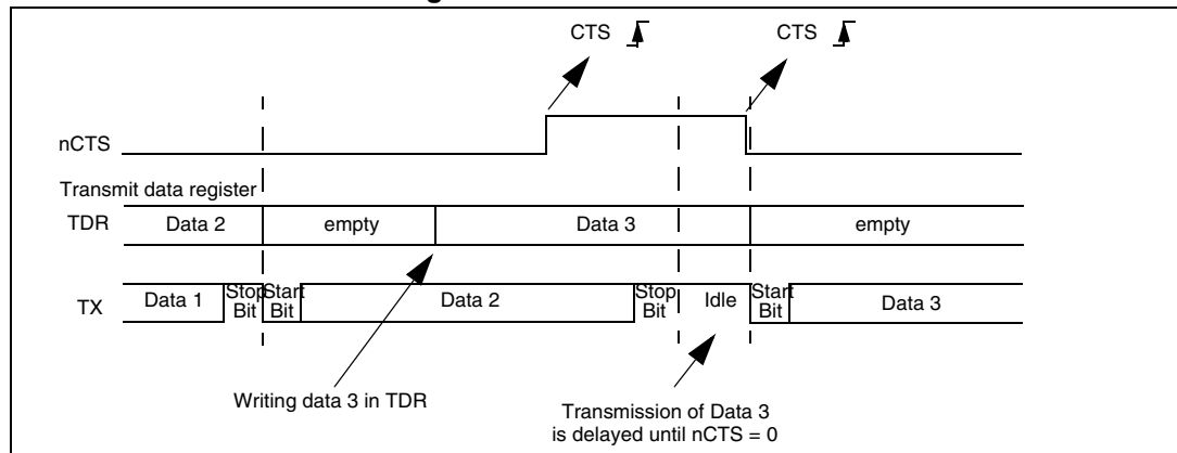
Figure 246. CTS flow control
