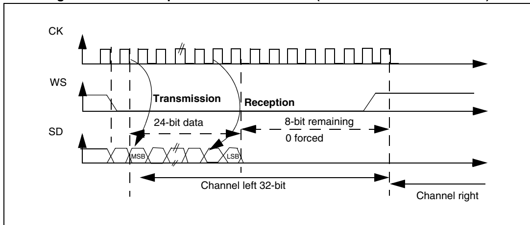
Figure 266. I 2 S Philips standard waveforms (24-bit frame with CPOL = 0)
