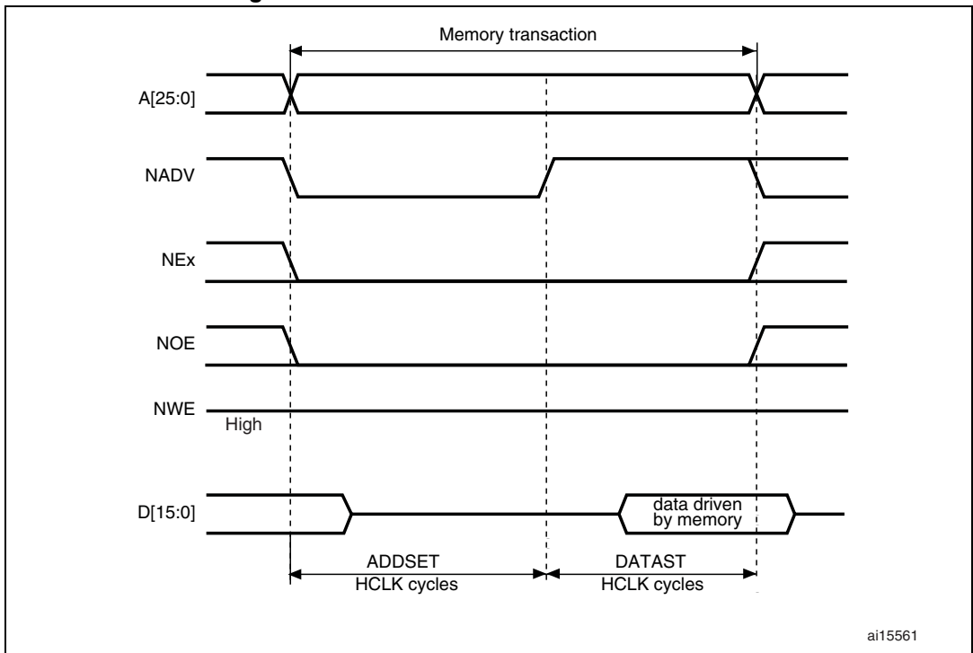
Figure 401. Mode2 and mode B read accesses
