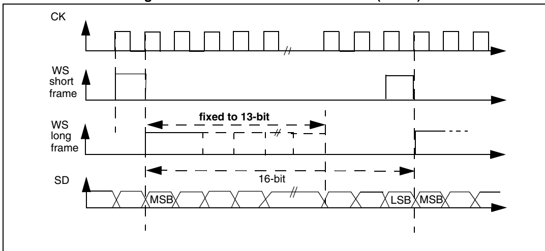
Figure 280. PCM standard waveforms (16-bit)
