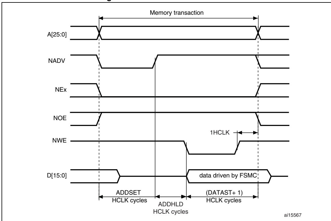
Figure 407. Mode D write accesses
