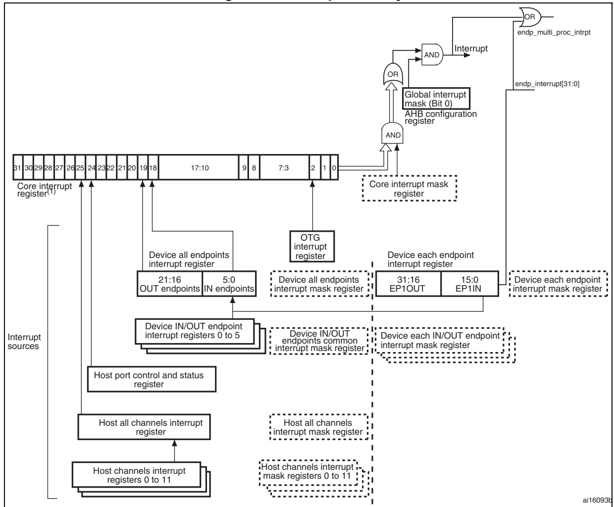
Figure 375. Interrupt hierarchy
