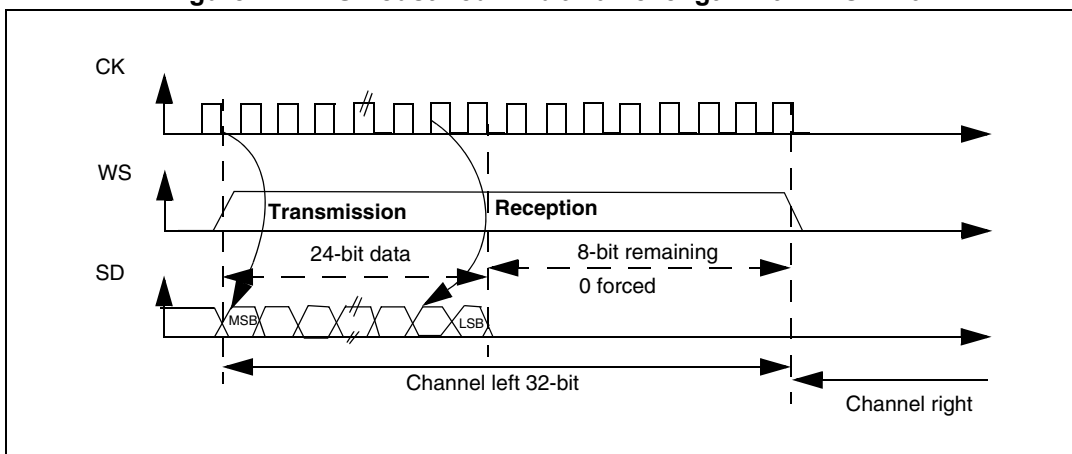
Figure 272. MSB Justified 24-bit frame length with CPOL = 0
