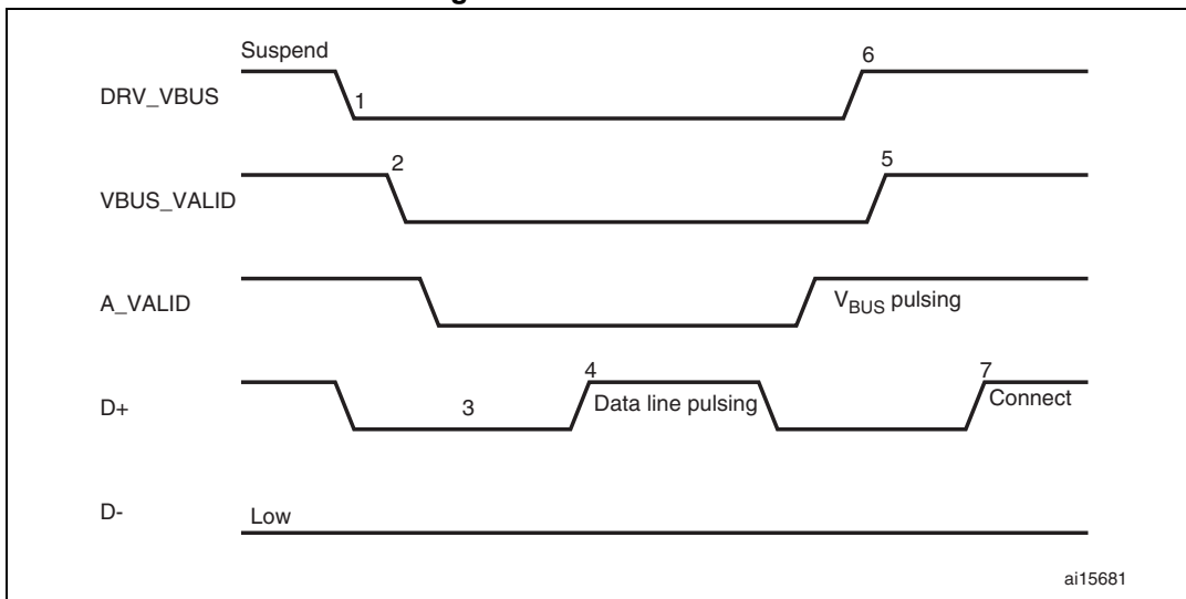
Figure 369. A-device SRP
