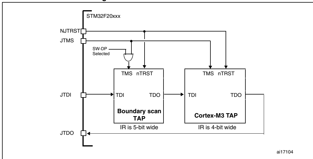
Figure 419. JTAG TAP connections
