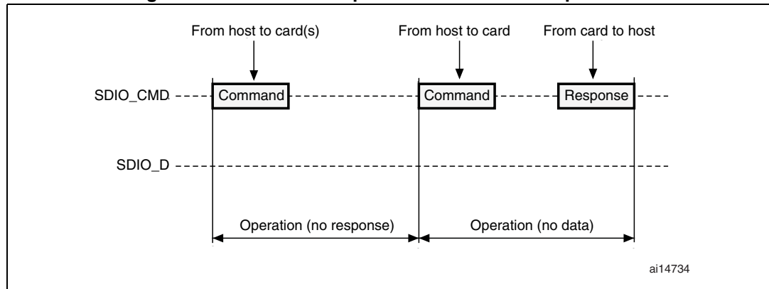
Figure 284. SDIO “no response” and “no data” operations
