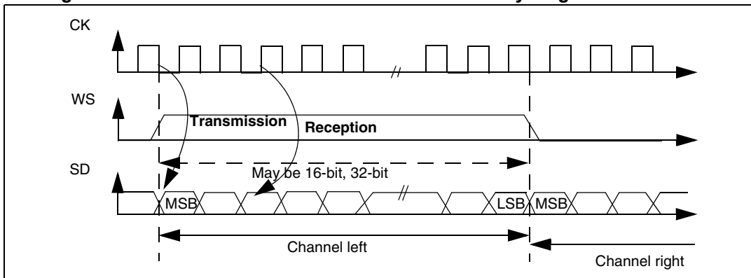
Figure 271. MSB Justified 16-bit or 32-bit full-accuracy length with CPOL = 0
