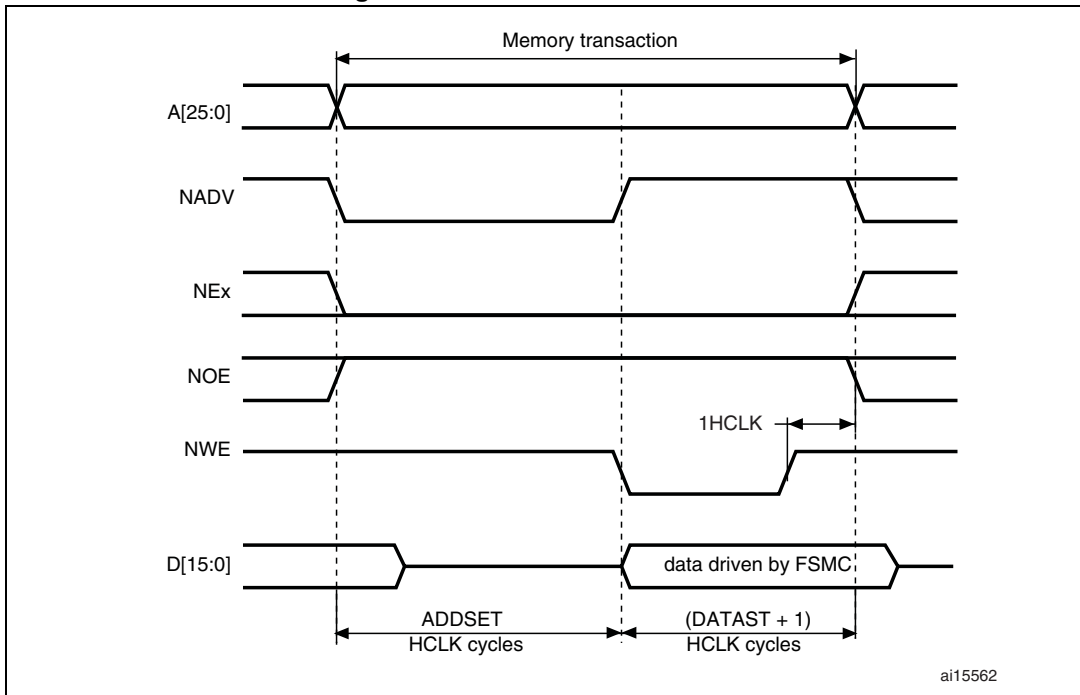
Figure 403. Mode B write accesses
