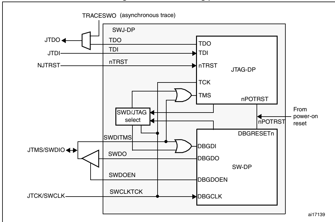
Figure 418 shows that the asynchronous TRACE output (TRACESWO) is multiplexed with TDO. This means that the asynchronous trace can only be used with SW-DP, not JTAG-DP.
