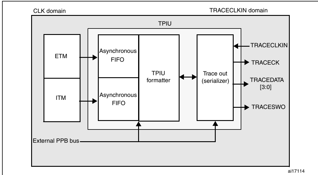
Figure 420. TPIU block diagram
