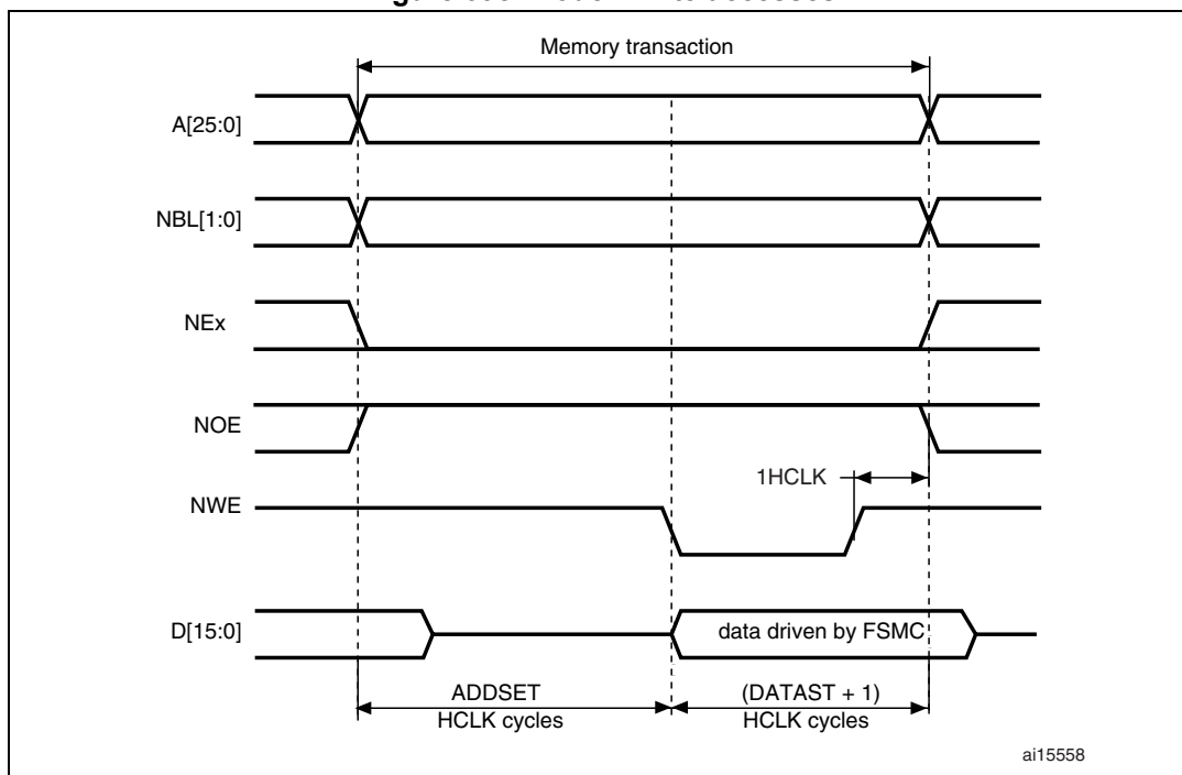
Figure 398. Mode1 write accesses
