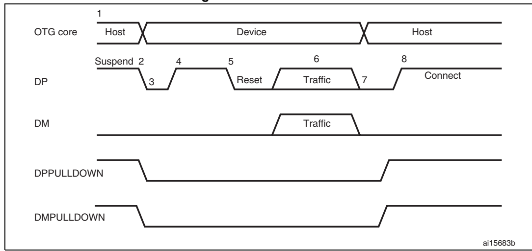
Figure 393. A-device HNP
