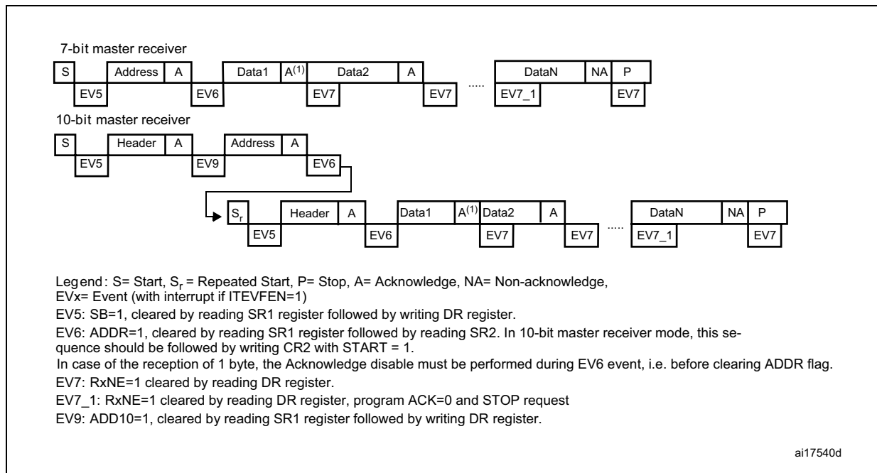
Figure 221. Transfer sequence diagram for master receiver
