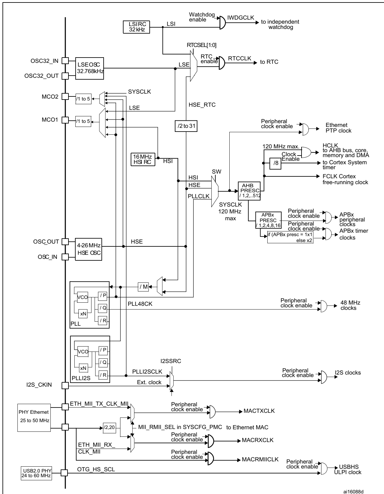
Figure 9. Clock tree
