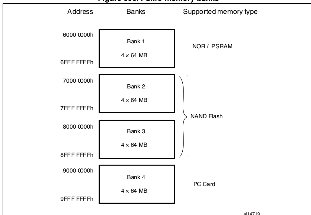
Figure 396. FSMC memory banks
