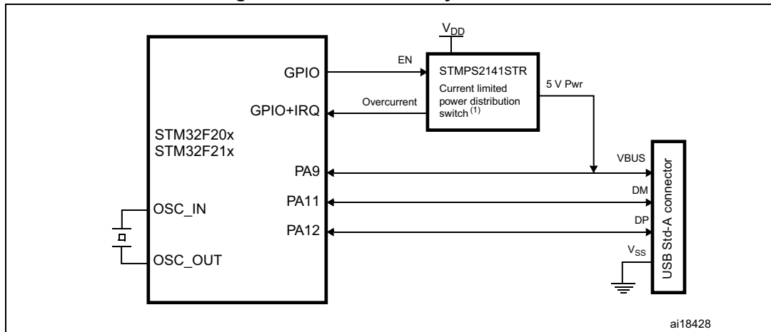
Figure 352. USB host-only connection
