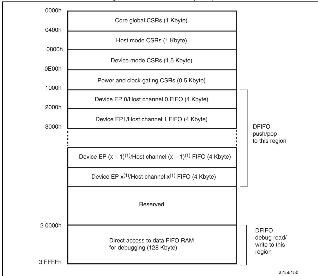
Figure 376. CSR memory map
