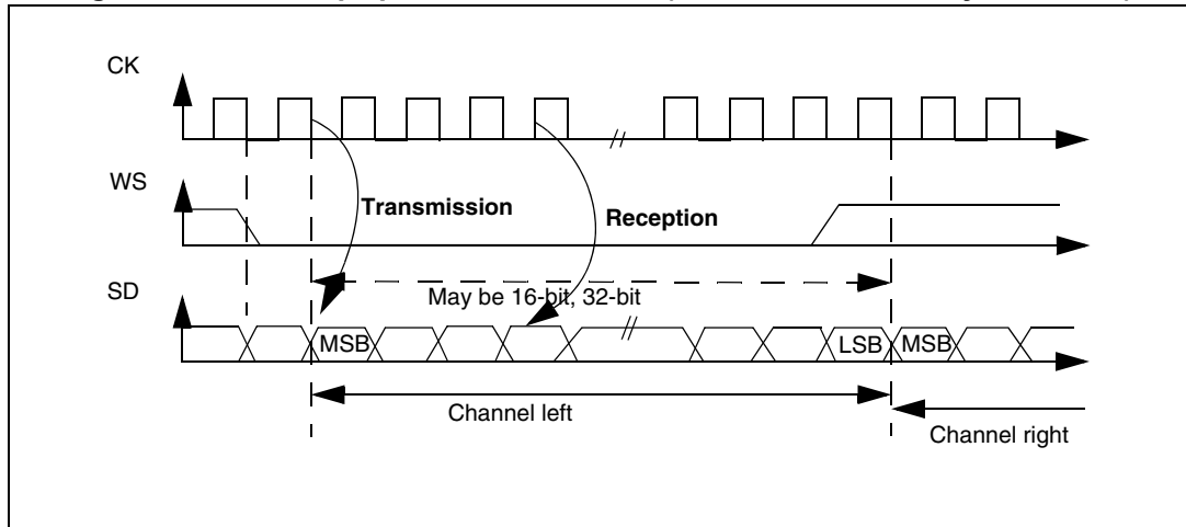
Figure 265. I 2 S Philips protocol waveforms (16/32-bit full accuracy, CPOL = 0)
