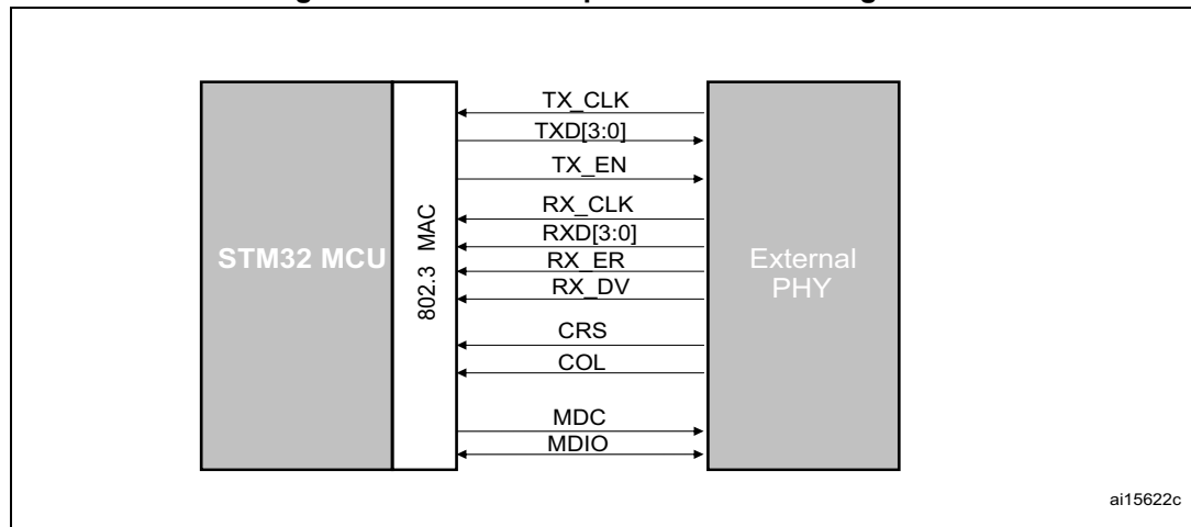
Figure 317. Media independent interface signals
