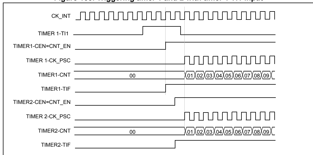
Figure 158. Triggering timer 1 and 2 with timer 1 T11 input
