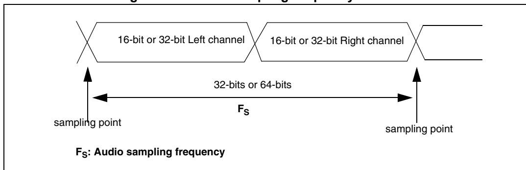
Figure 282. Audio sampling frequency definition
