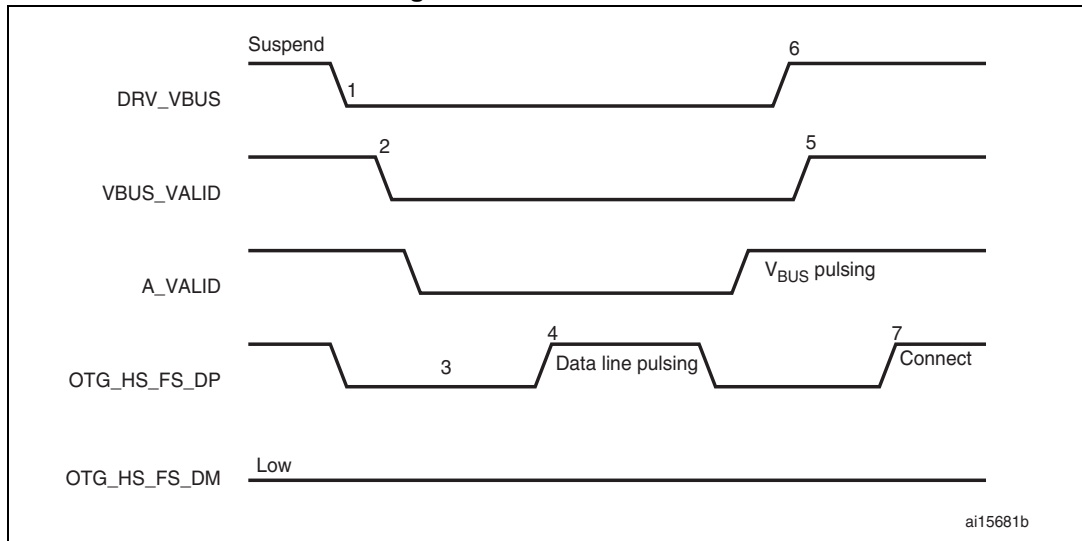
Figure 391. A-device SRP
