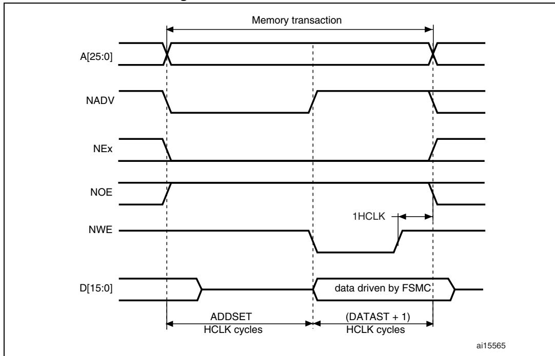
Figure 405. Mode C write accesses
