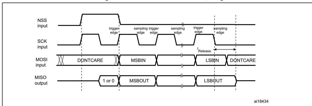
Figure 251. TI mode - Slave mode, single transfer
