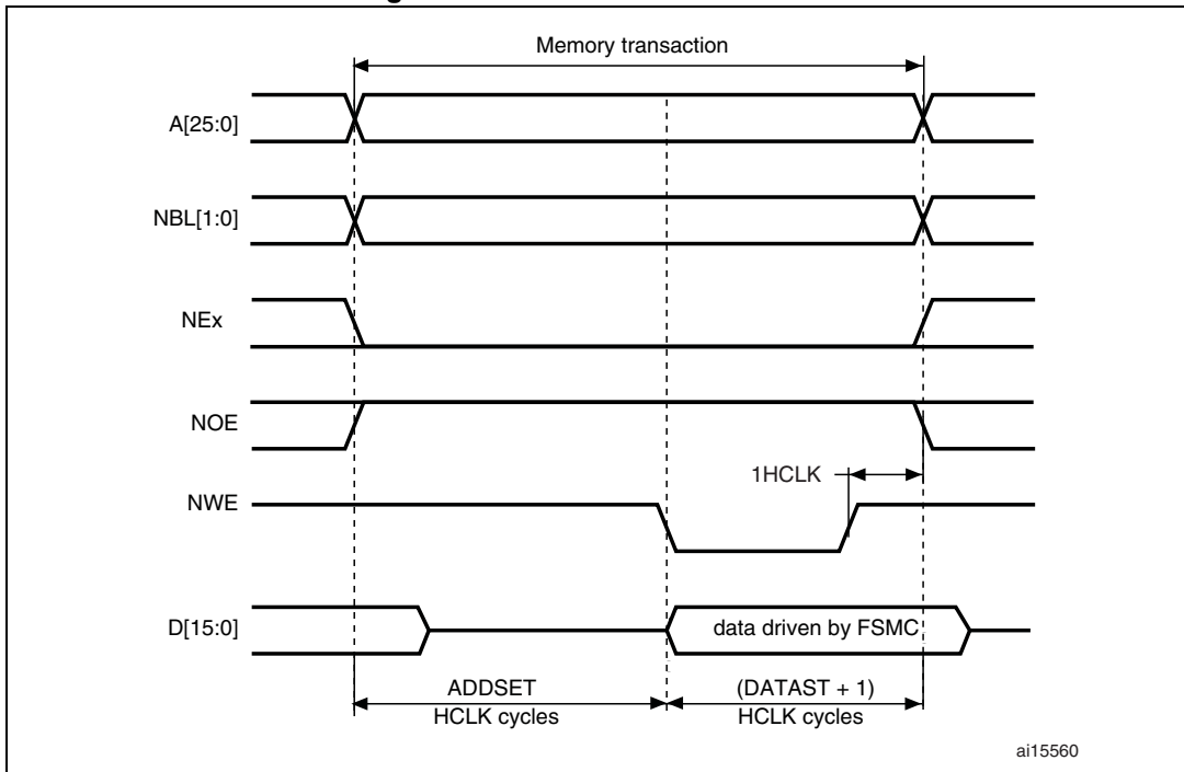
Figure 400. ModeA write accesses
