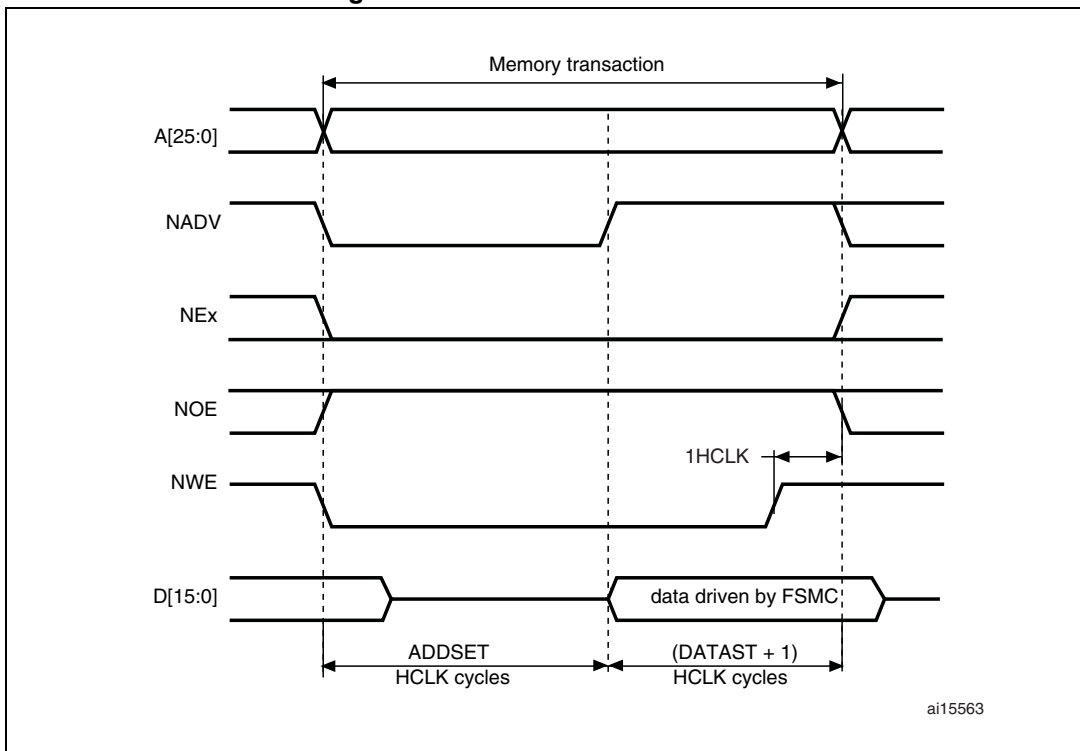
Figure 403. Mode B write accesses
