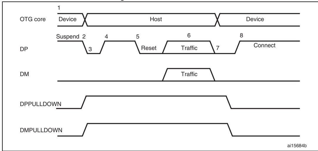
Figure 394. B-device HNP
