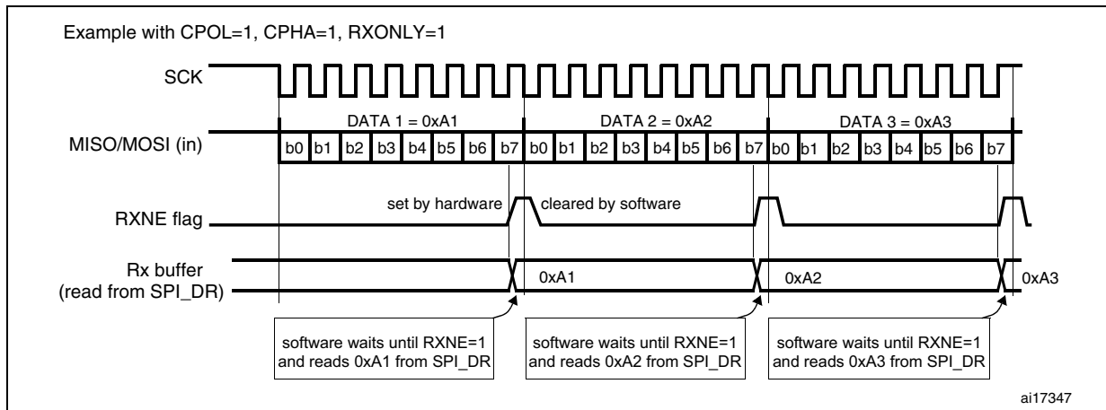
Figure 259. RXNE behavior in receive-only mode (BIDIRMODE=0 and RXONLY=1) in the case of continuous transfers
