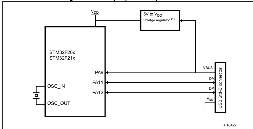
Figure 351. USB peripheral-only connection
