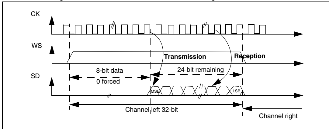
Figure 275. LSB Justified 24-bit frame length with CPOL = 0
