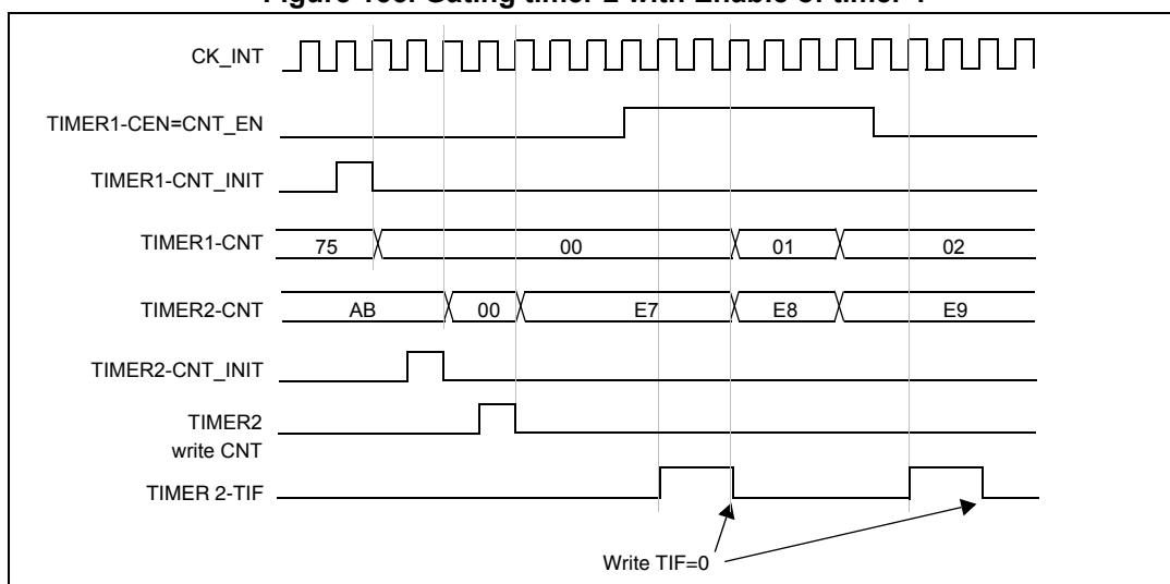
Figure 155. Gating timer 2 with Enable of timer 1
