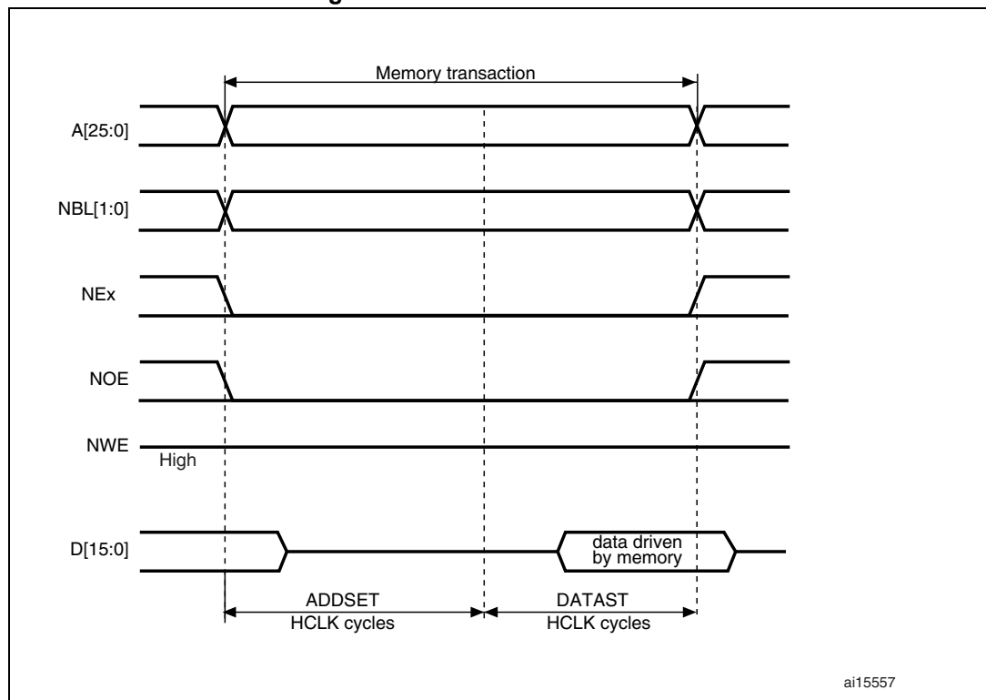
Figure 397. Mode1 read accesses
