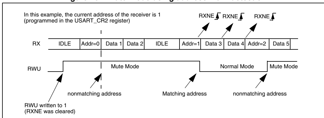
Figure 231. Mute mode using address mark detection
