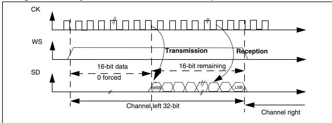
Figure 278. LSB justified 16-bit extended to 32-bit packet frame with CPOL = 0
