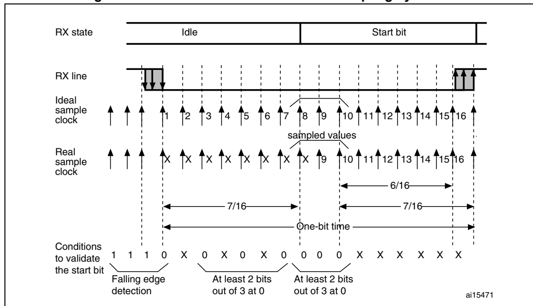
Figure 227. Start bit detection when oversampling by 16 or 8
