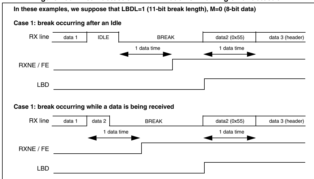
Figure 233. Break detection in LIN mode vs. Framing error detection
