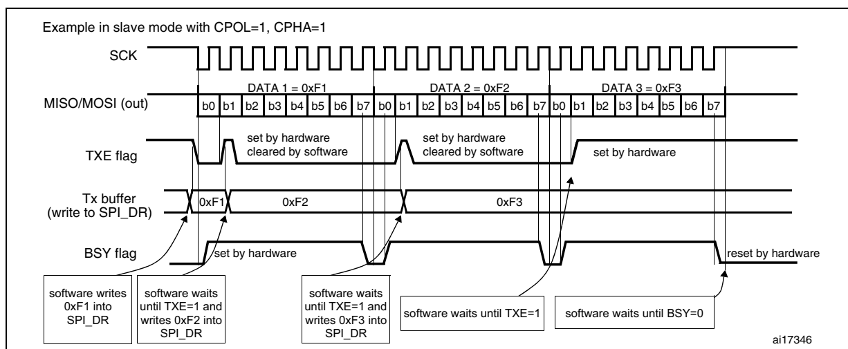
Figure 258. TXE/BSY in Slave transmit-only mode (BIDIMODE=0 and RXONLY=0) in the case of continuous transfers
