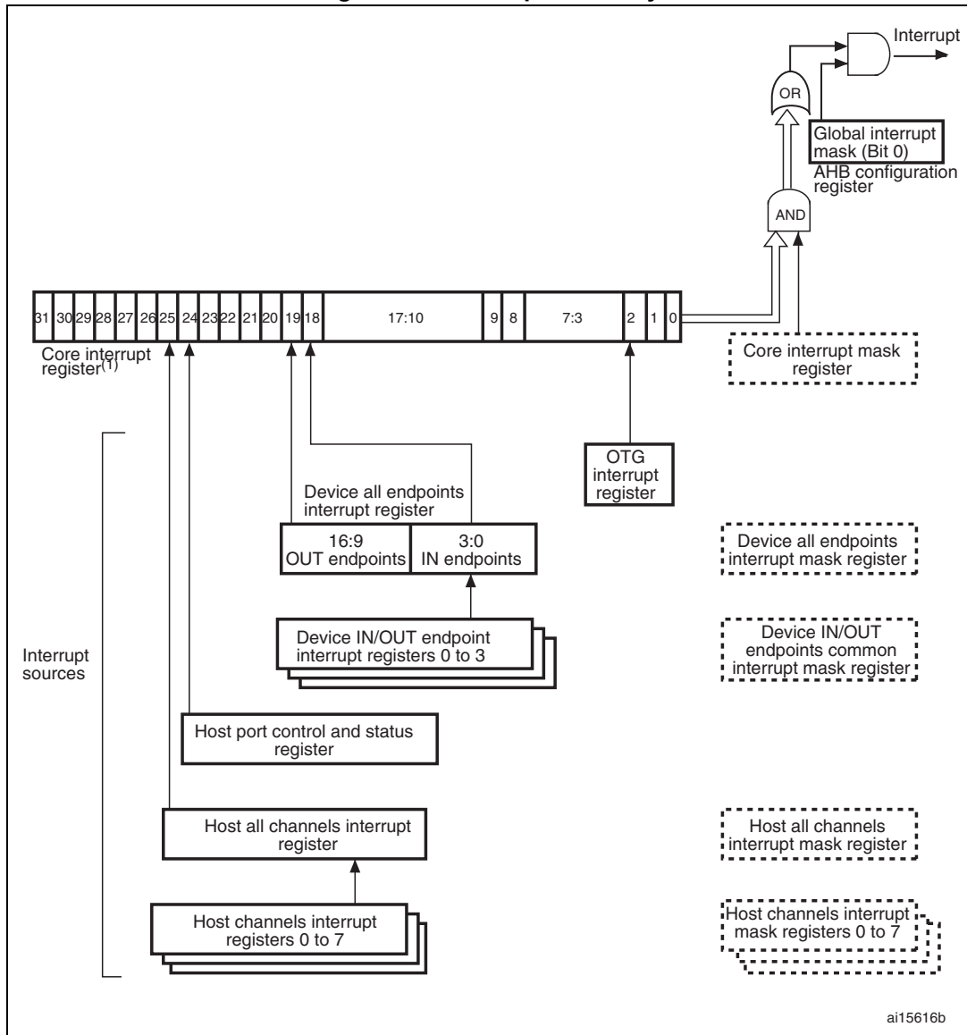
Figure 357. Interrupt hierarchy
