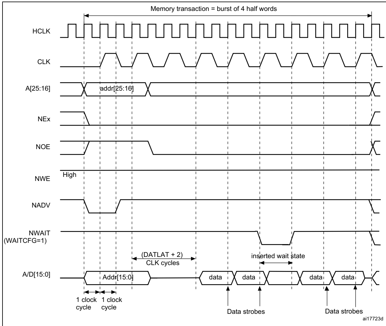
Figure 413. Synchronous multiplexed read mode - NOR, PSRAM (CRAM)
