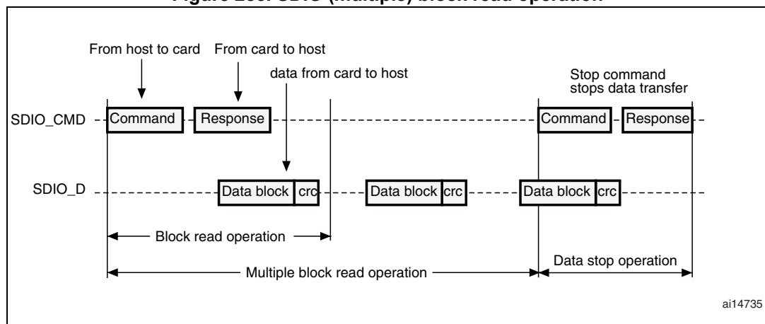
Figure 285. SDIO (multiple) block read operation
