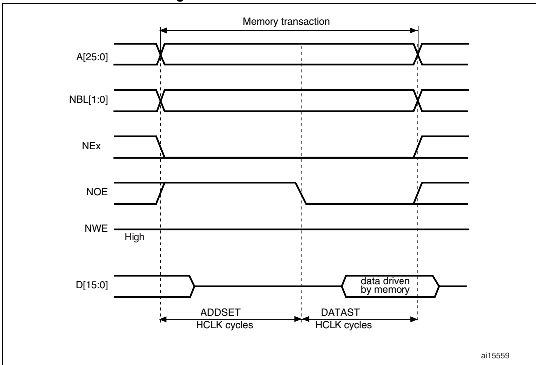
Figure 399. ModeA read accesses
