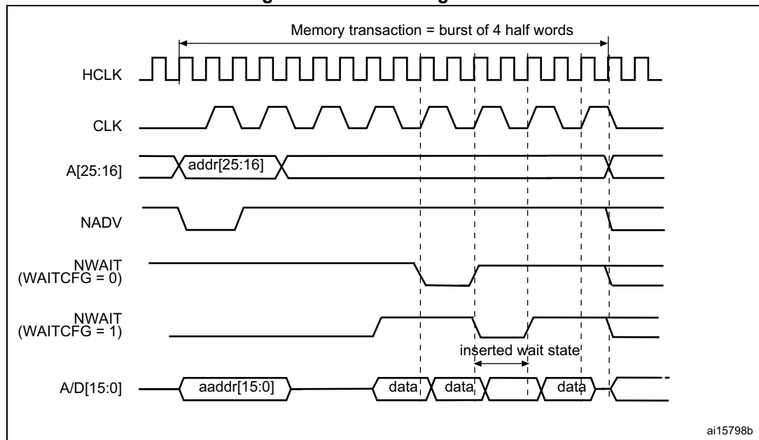
Figure 412. Wait configurations
