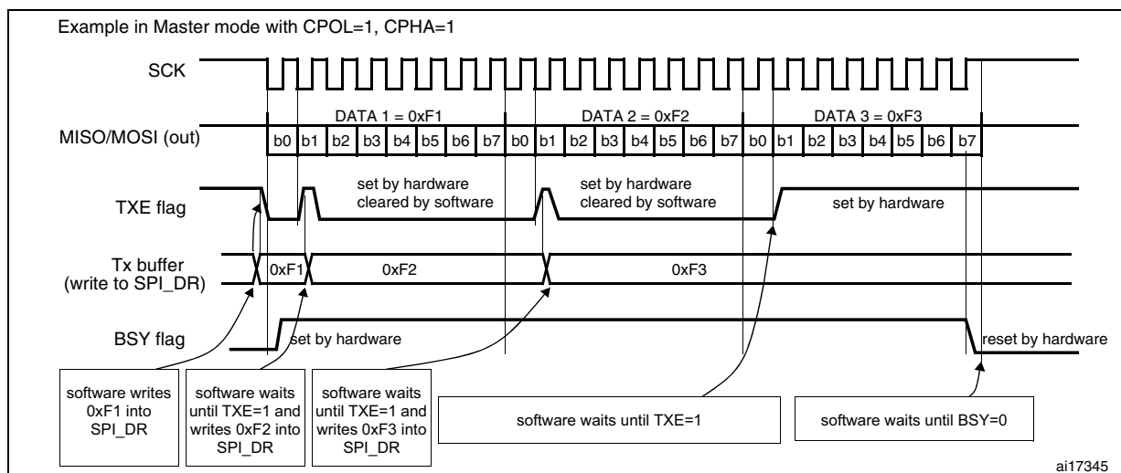
Figure 257. TXE/BSY behavior in Master transmit-only mode (BIDIMODE=0 and RXONLY=0) in case of continuous transfers
