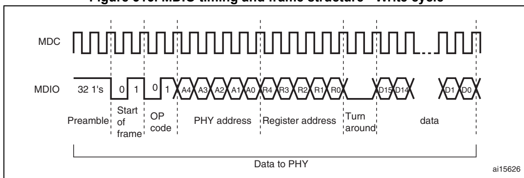
Figure 315. MDIO timing and frame structure - Write cycle
