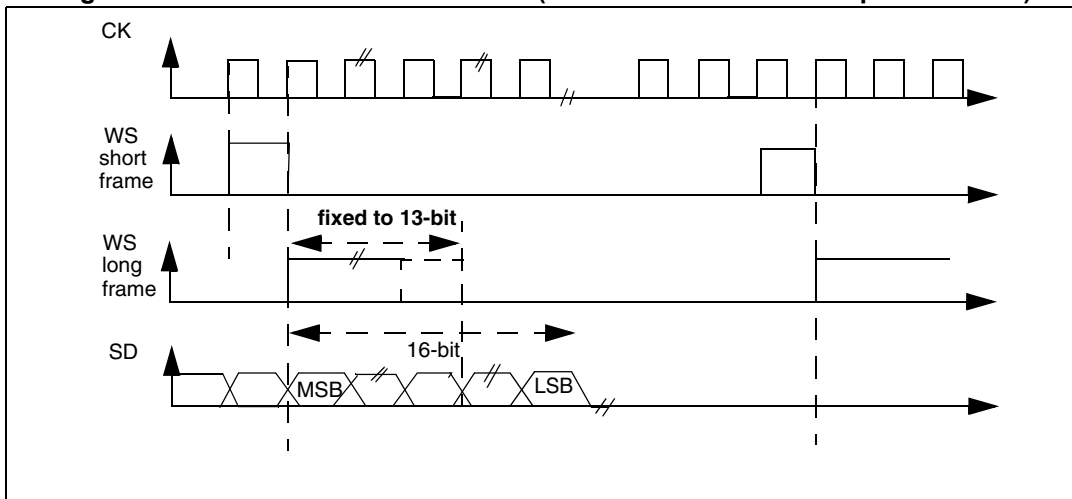
Figure 281. PCM standard waveforms (16-bit extended to 32-bit packet frame)
