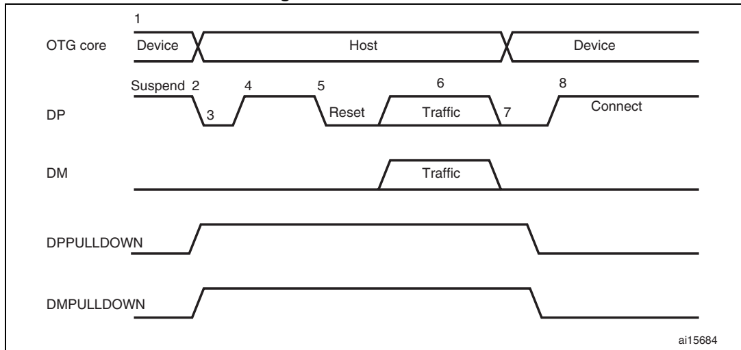
Figure 372. B-device HNP
