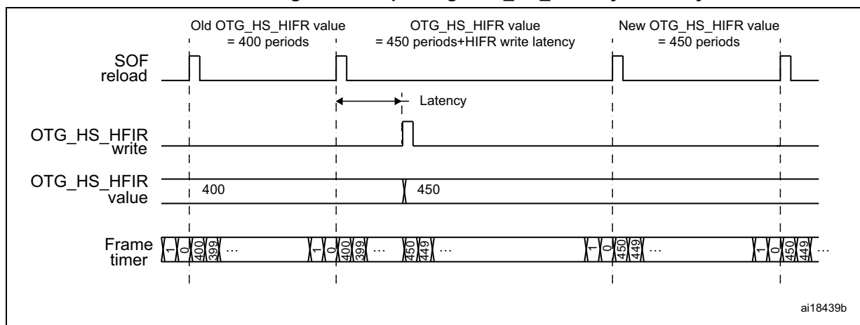
Figure 374. Updating OTG_HS_HFIR dynamically
