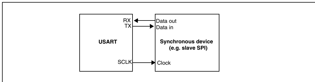
Figure 234. USART example of synchronous transmission
