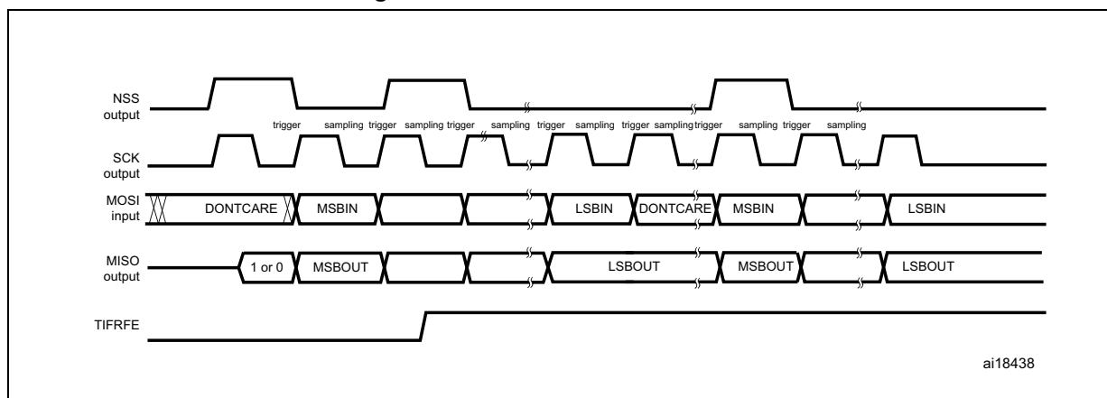
Figure 263. TI mode frame format error detection
