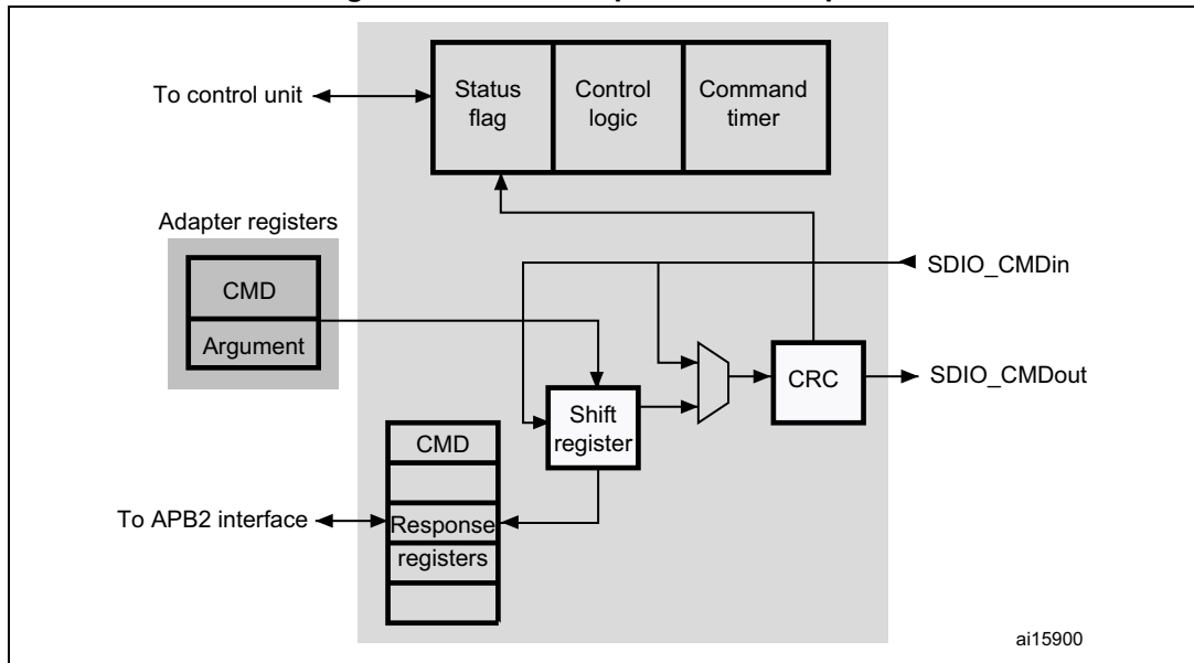
Figure 292. SDIO adapter command path
