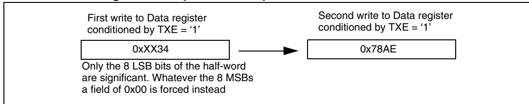
Figure 276. Operations required to transmit 0x3478AE
