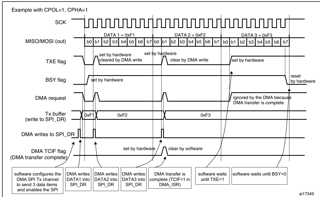
Figure 261. Transmission using DMA
