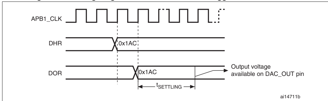
Figure 67. Timing diagram for conversion with trigger disabled TEN = 0
