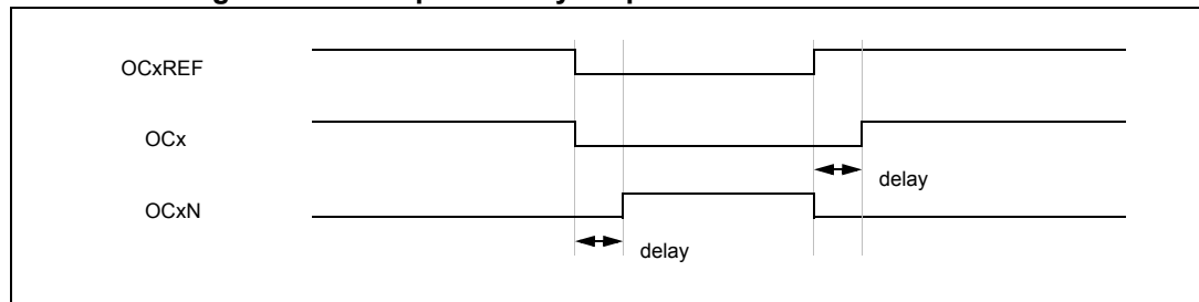
Figure 120. Complementary output with dead-time insertion.
