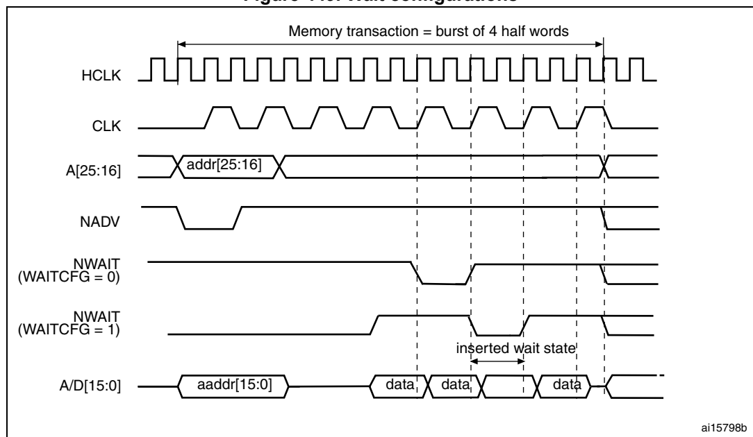
Figure 449. Wait configurations
