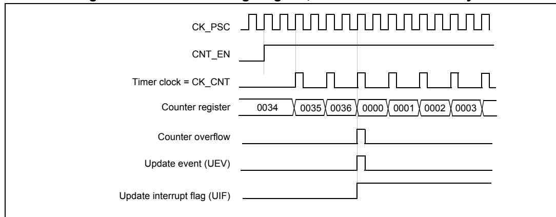
Figure 185. Counter timing diagram, internal clock divided by 2
