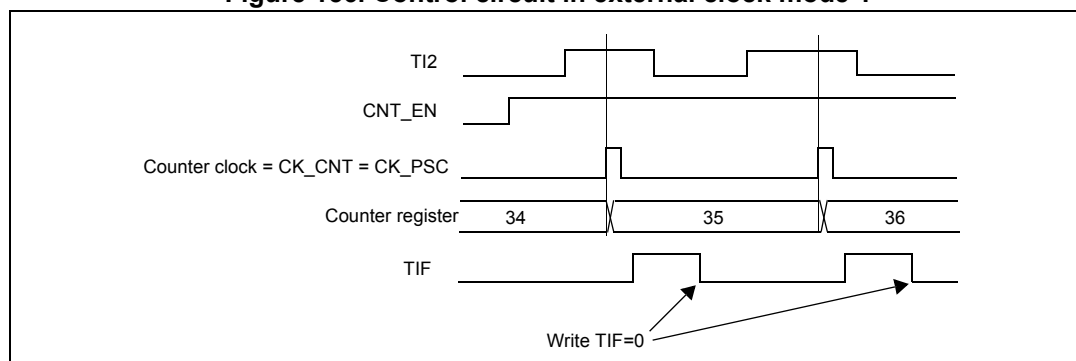
Figure 156. Control circuit in external clock mode 1
