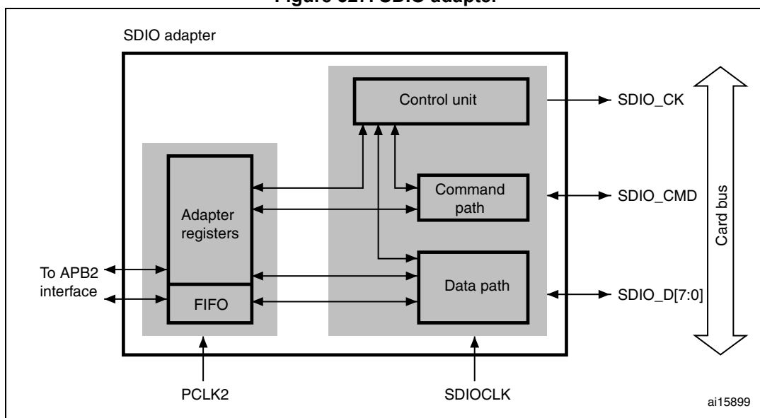
Figure 327. SDIO adapter
