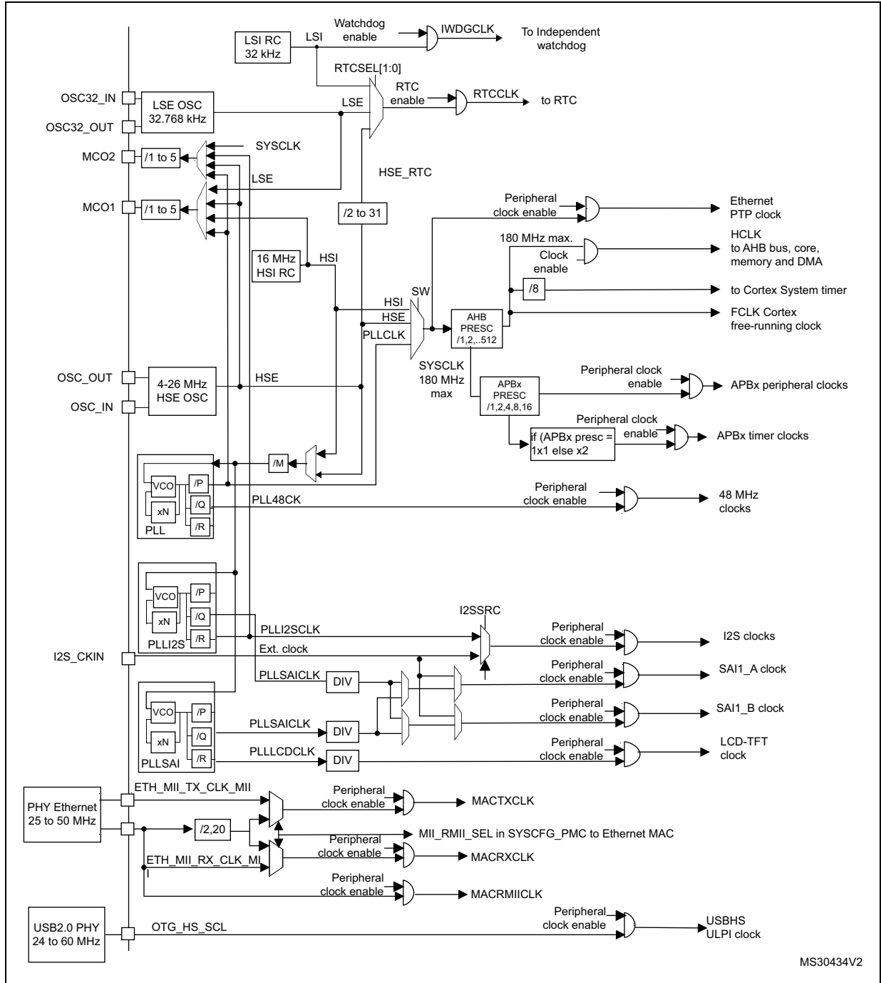
Figure 16. Clock tree
