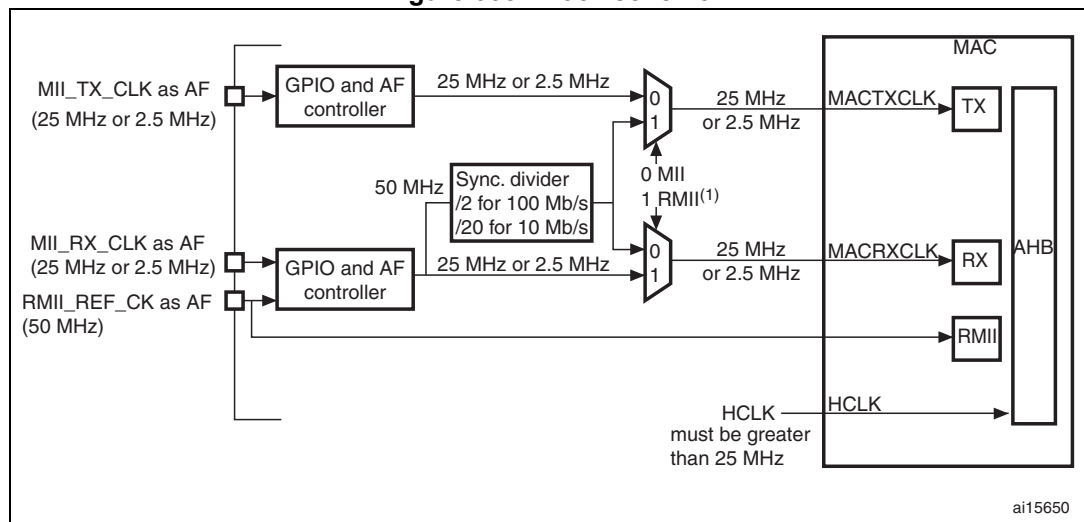
Figure 358. Clock scheme
