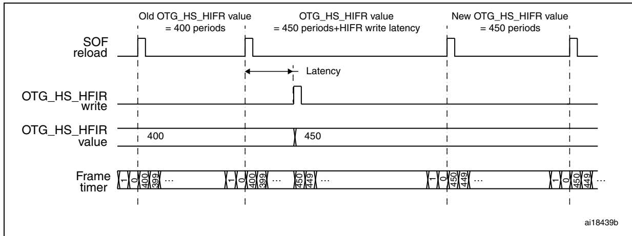
Figure 411. Updating OTG_HS_HFIR dynamically
