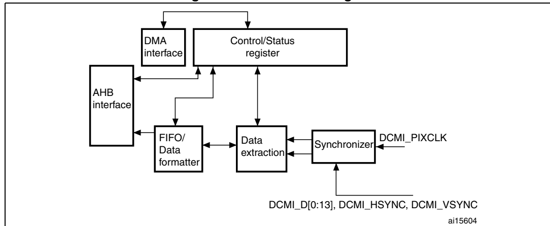
Figure 73. Top-level block diagram
