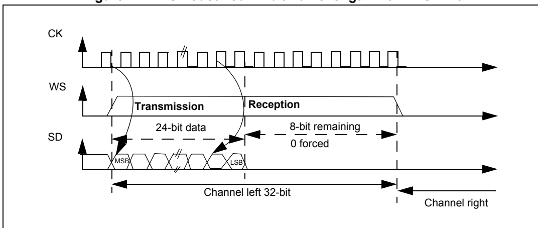
Figure 271. MSB Justified 24-bit frame length with CPOL = 0
