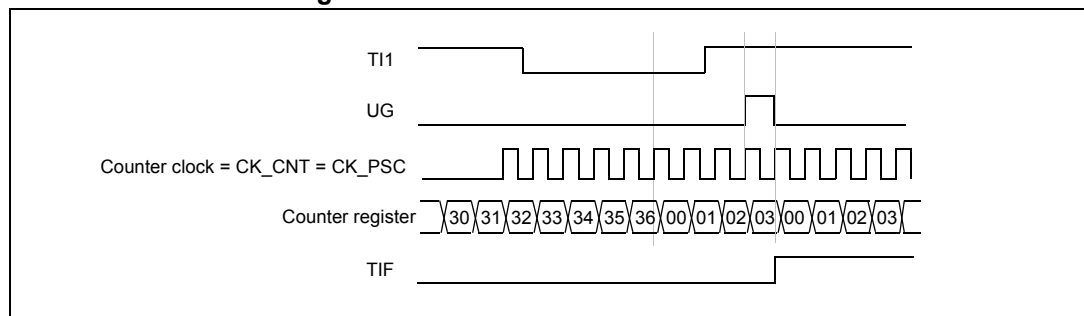
Figure 170. Control circuit in reset mode
