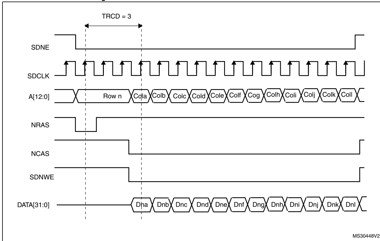
Figure 476. Burst write SDRAM access waveforms
