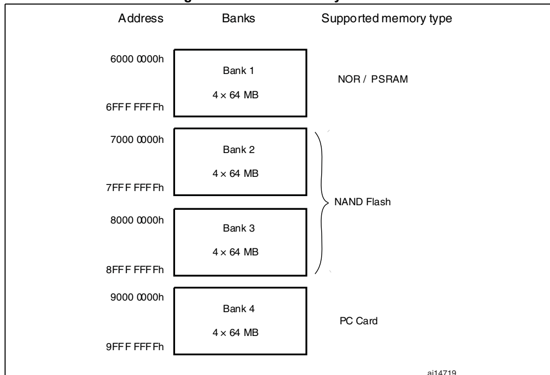
Figure 433. FSMC memory banks
