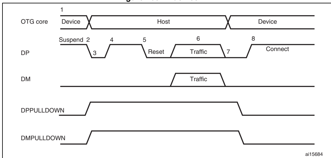
Figure 409. B-device HNP
