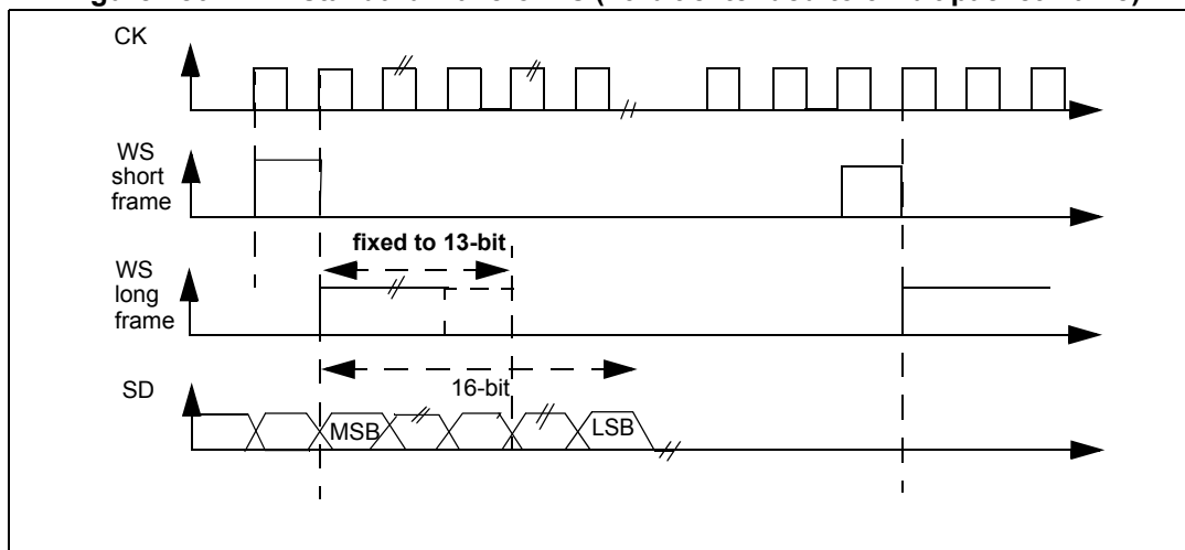
Figure 280. PCM standard waveforms (16-bit extended to 32-bit packet frame)
