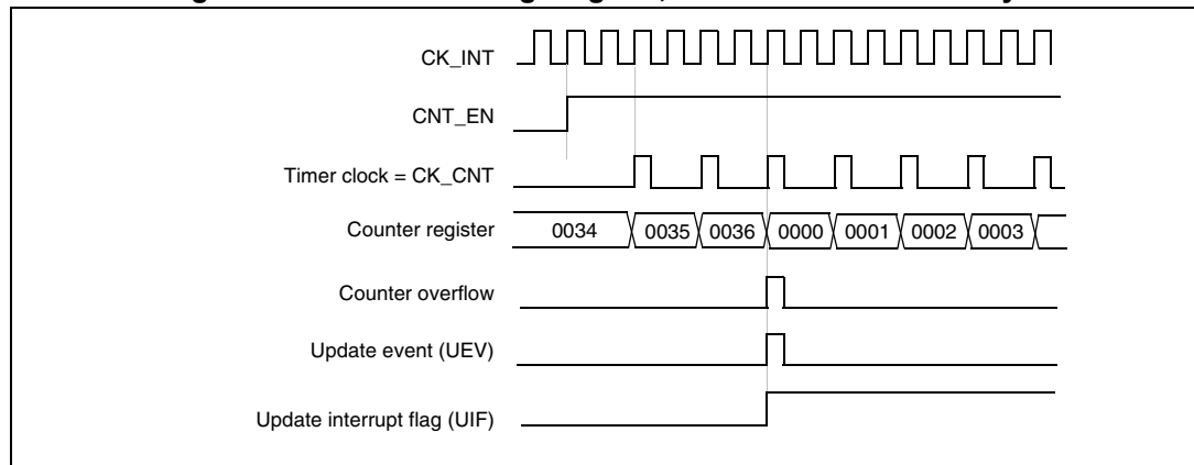
Figure 207. Counter timing diagram, internal clock divided by 2
