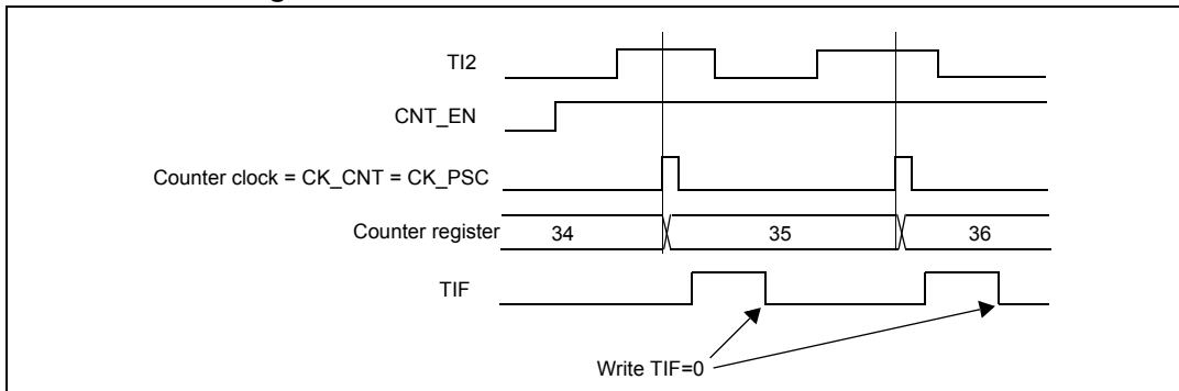
Figure 192. Control circuit in external clock mode 1
