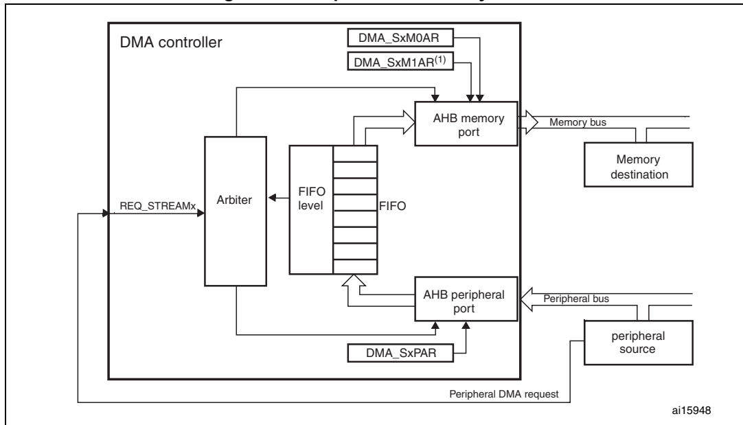
Figure 36. Peripheral-to-memory mode
