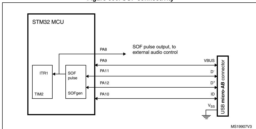
Figure 390. SOF connectivity
