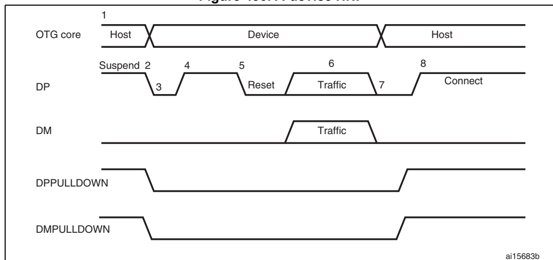
Figure 430. A-device HNP
