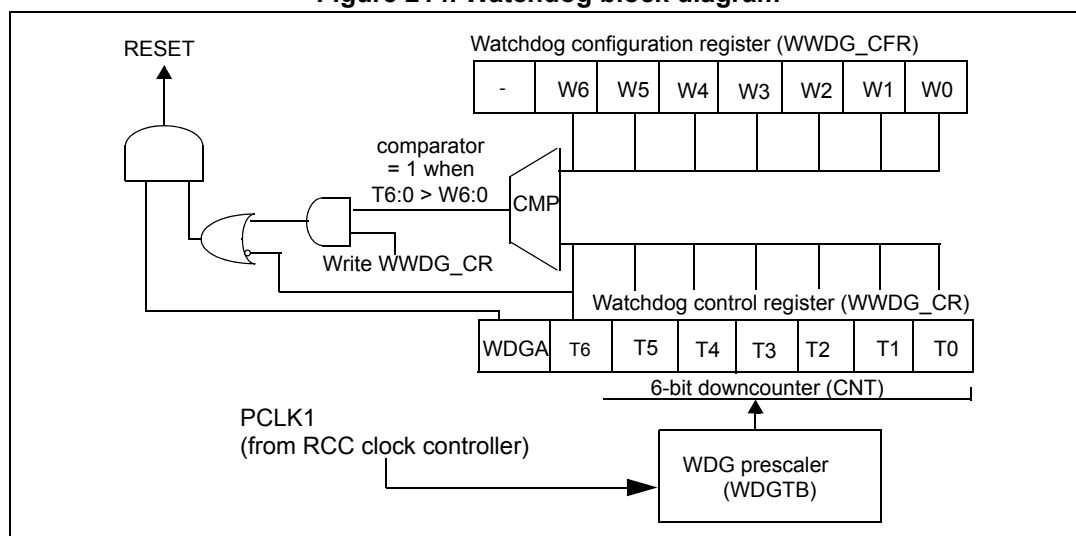
Figure 214. Watchdog block diagram
