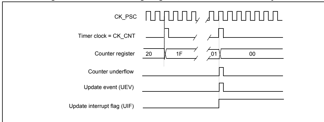
Figure 103. Counter timing diagram, internal clock divided by N
