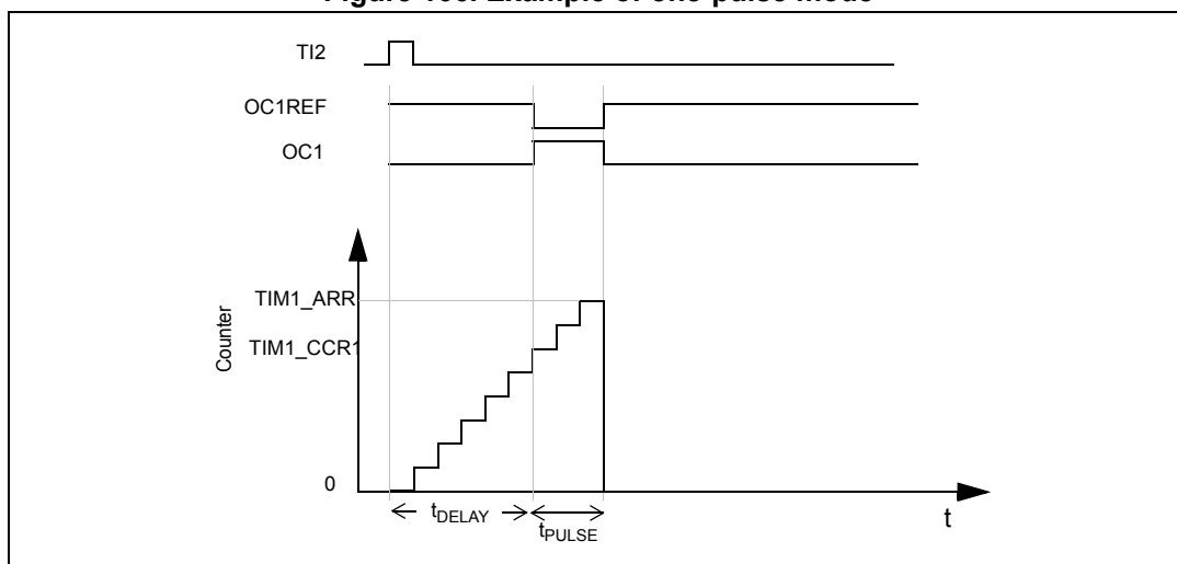
Figure 166. Example of one-pulse mode
