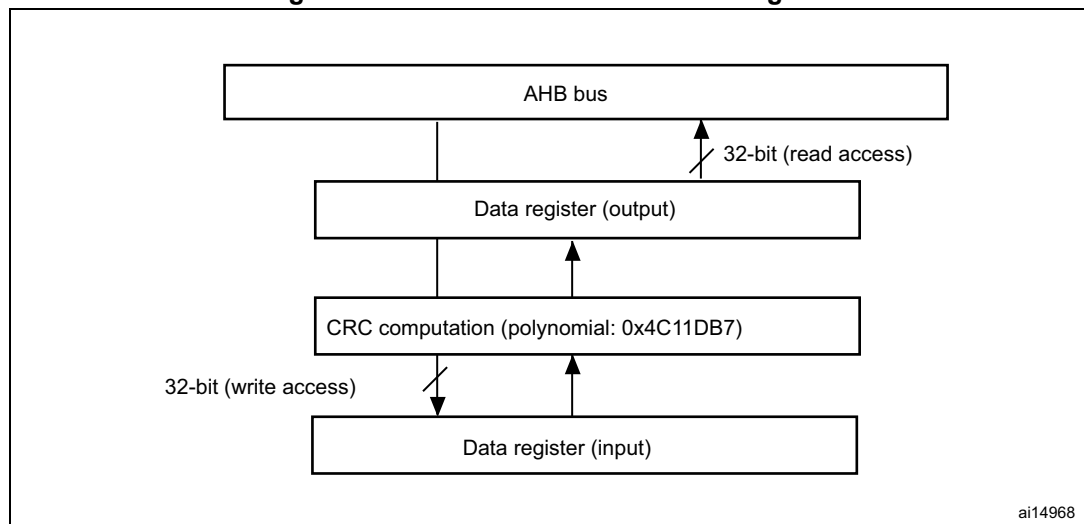
Figure 8. CRC calculation unit block diagram
