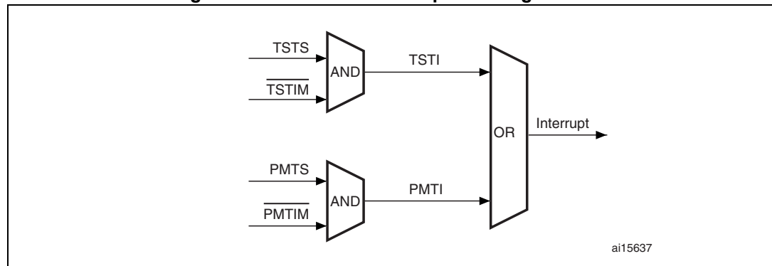
Figure 370. MAC core interrupt masking scheme
