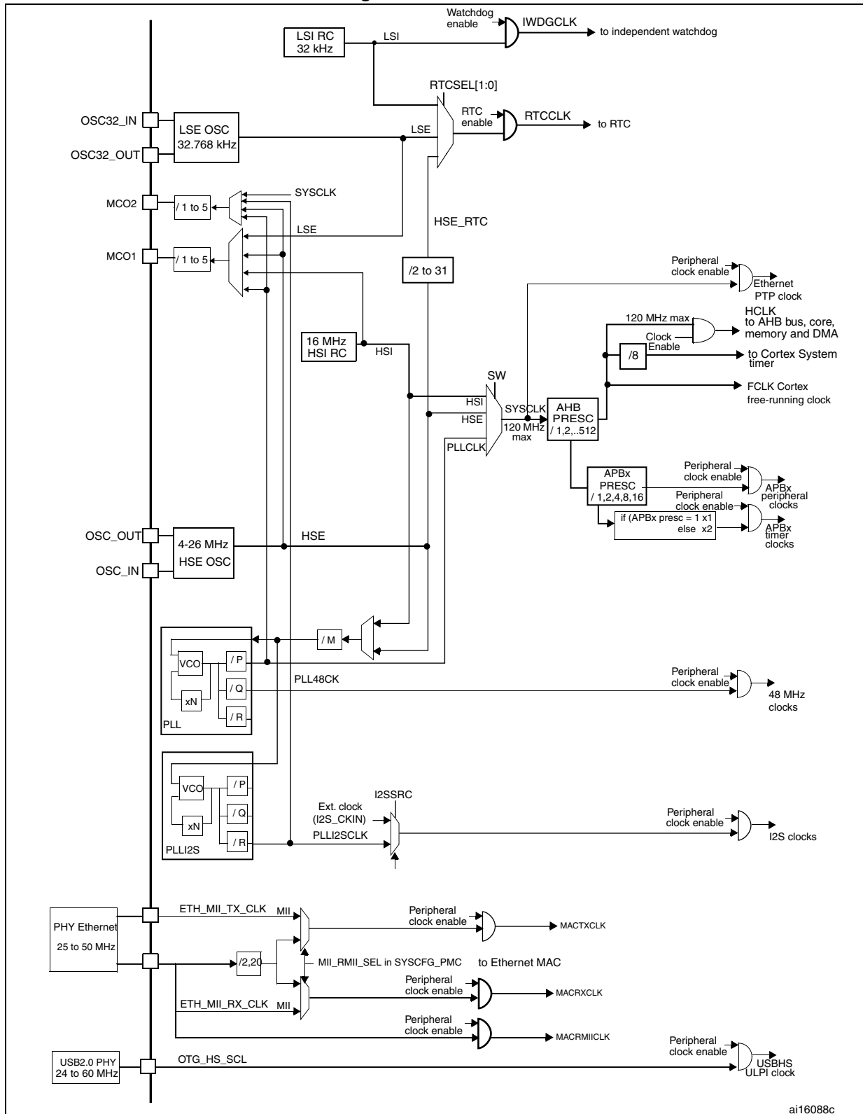
Figure 21. Clock tree
