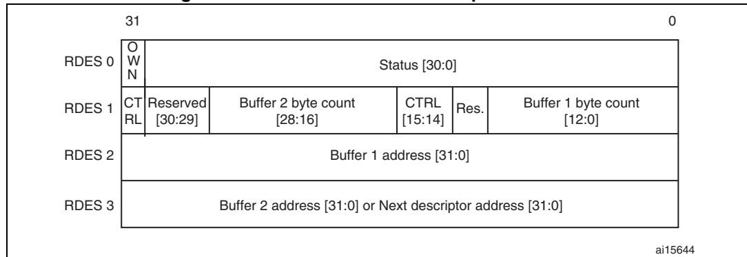
Figure 382. Normal Rx DMA descriptor structure
