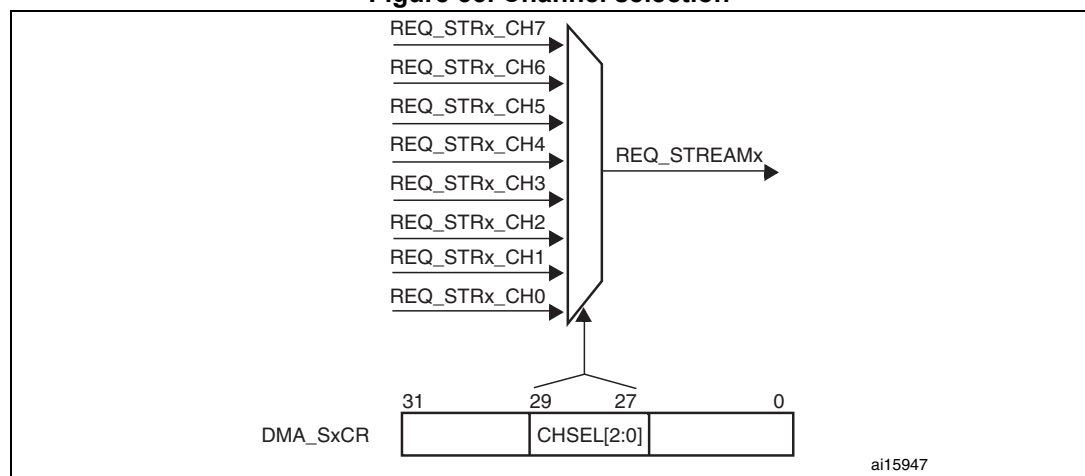
Figure 35. Channel selection
