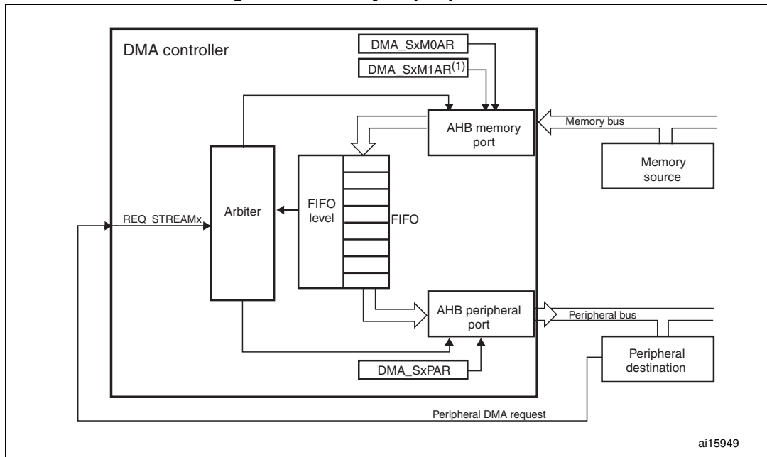
Figure 37. Memory-to-peripheral mode
