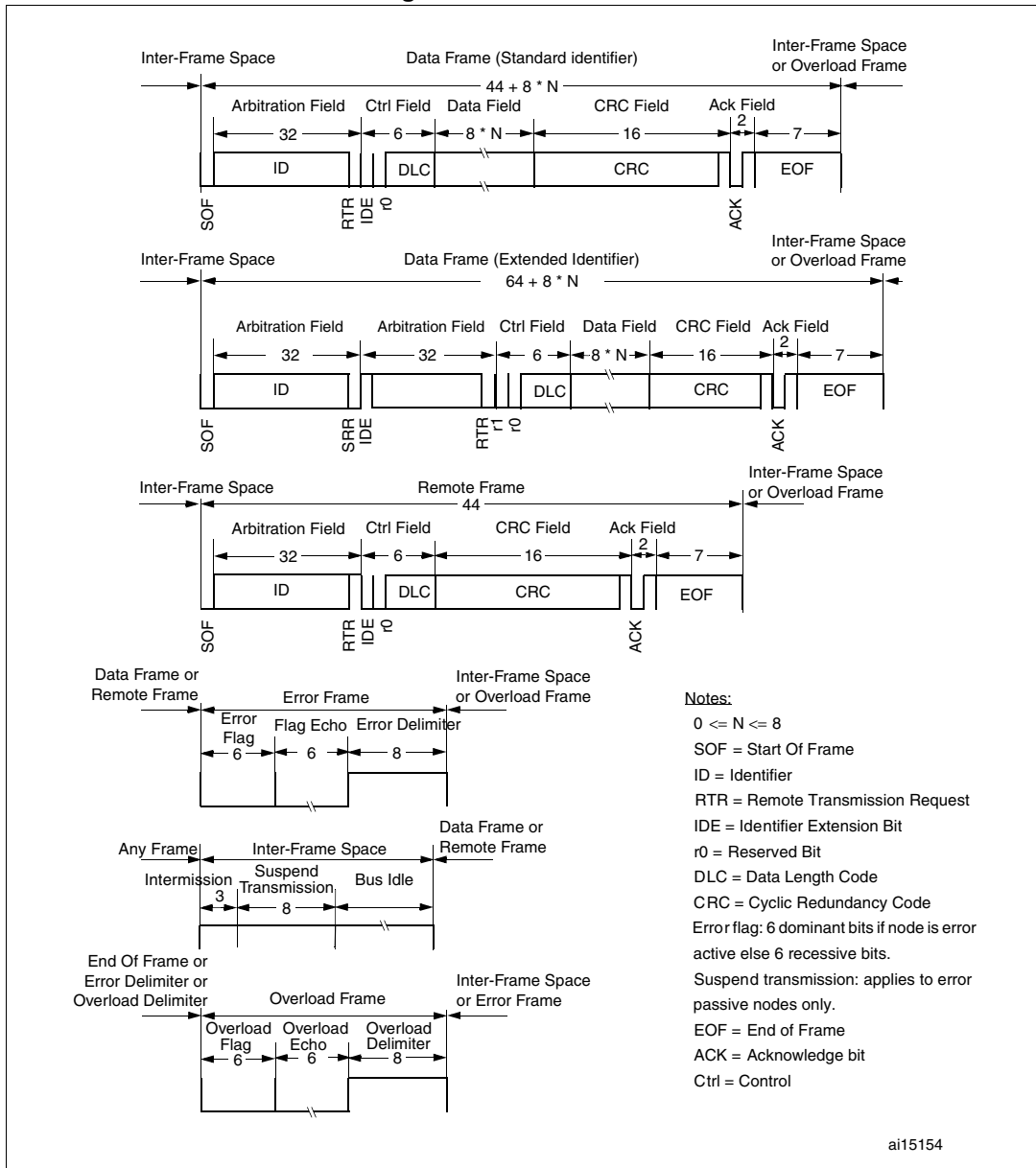
Figure 347. CAN frames
