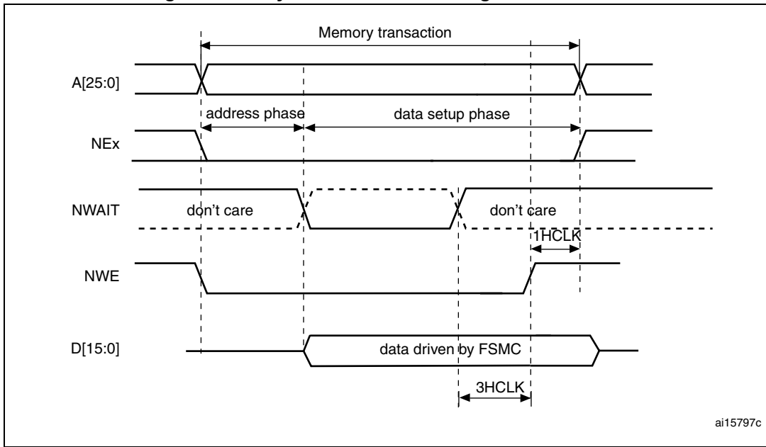
Figure 448. Asynchronous wait during a write access
