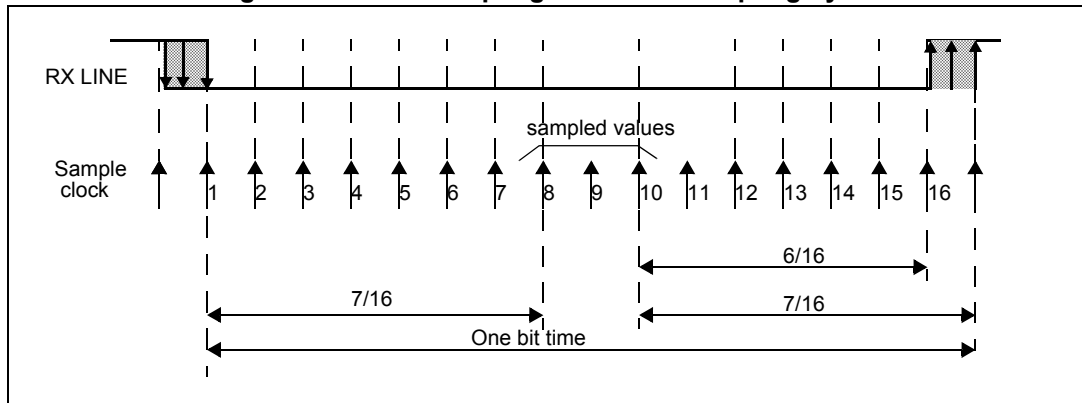
Figure 301. Data sampling when oversampling by 16
