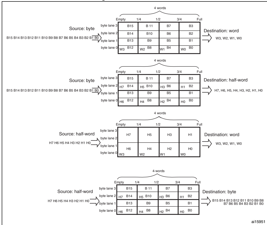
Figure 39. FIFO structure
