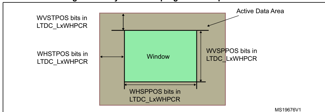
Figure 83. Layer window programmable parameters:
