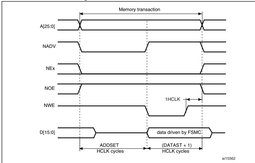
Figure 440. Mode B write accesses
