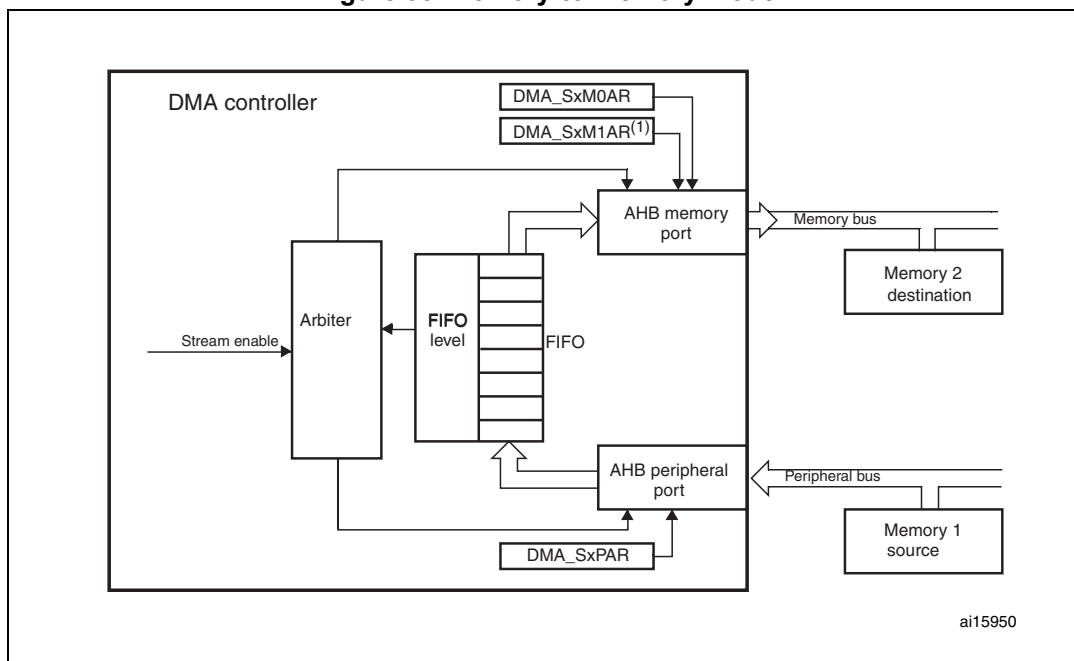
Figure 38. Memory-to-memory mode
