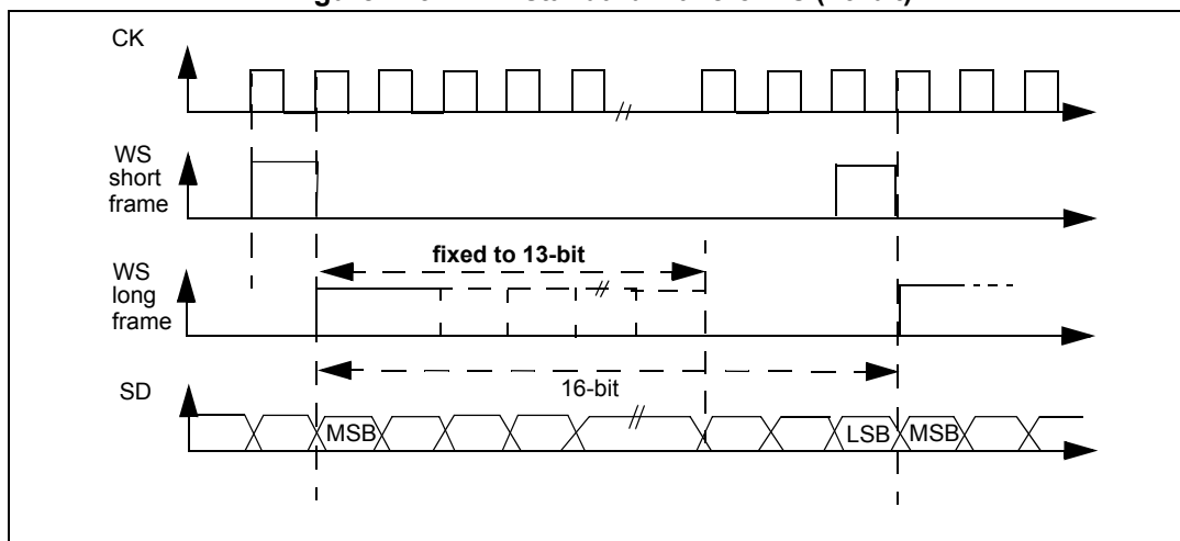
Figure 279. PCM standard waveforms (16-bit)
