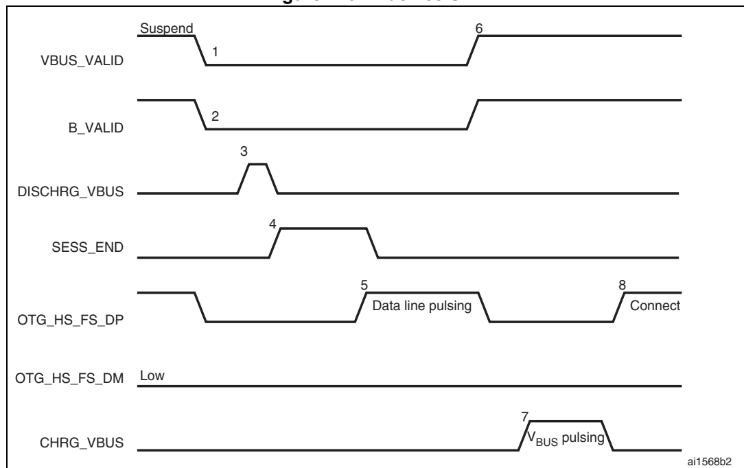
Figure 429. B-device SRP
