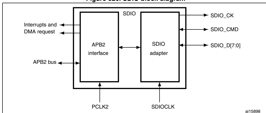
Figure 326. SDIO block diagram
