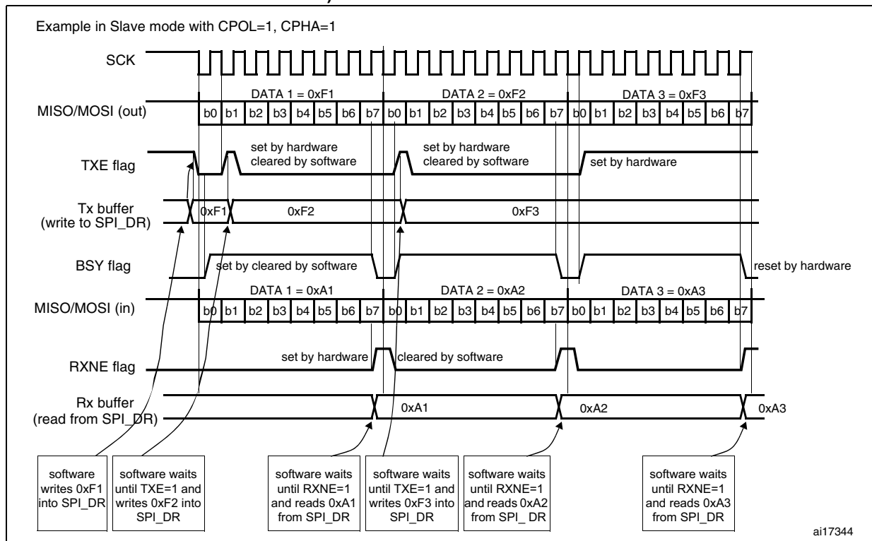
Figure 254. TXE/RXNE/BSY behavior in Slave / full-duplex mode (BIDIMODE=0, RXONLY=0) in the case of continuous transfers
