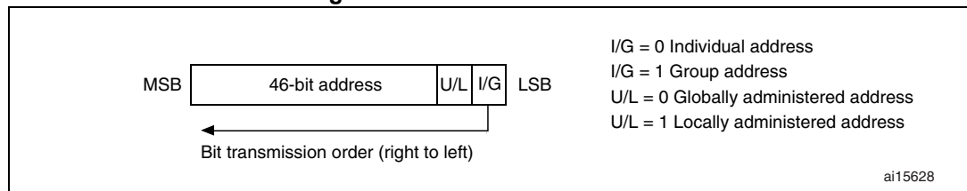
Figure 359. Address field format
