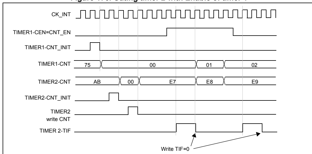
Figure 176. Gating timer 2 with Enable of timer 1
