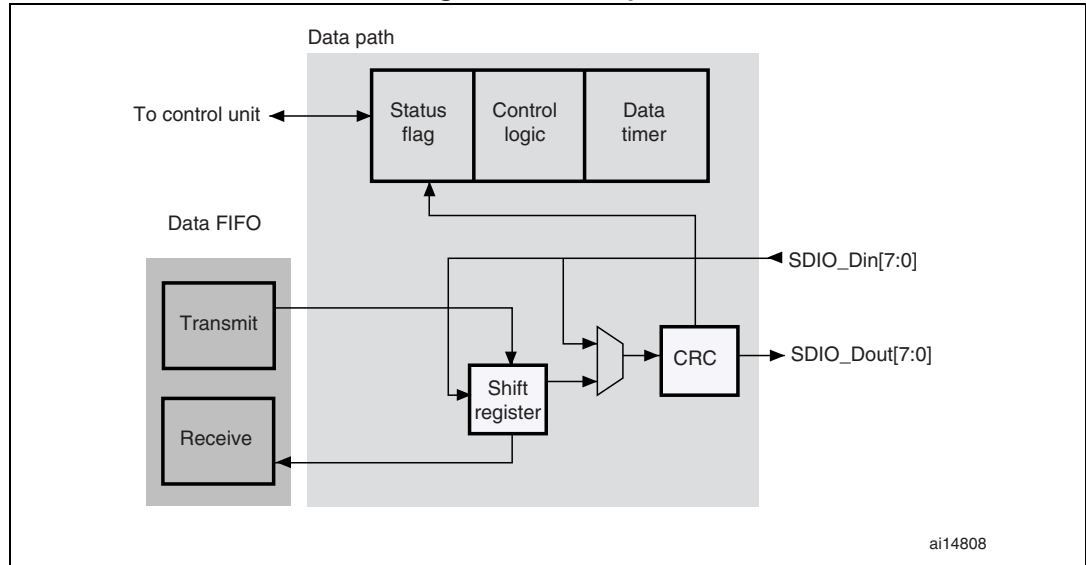
Figure 332. Data path
