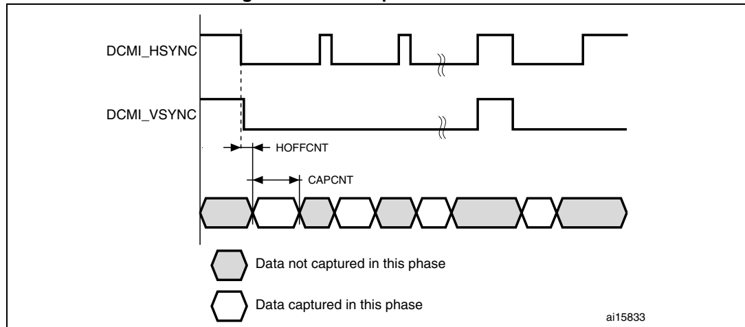
Figure 79. Data capture waveforms
