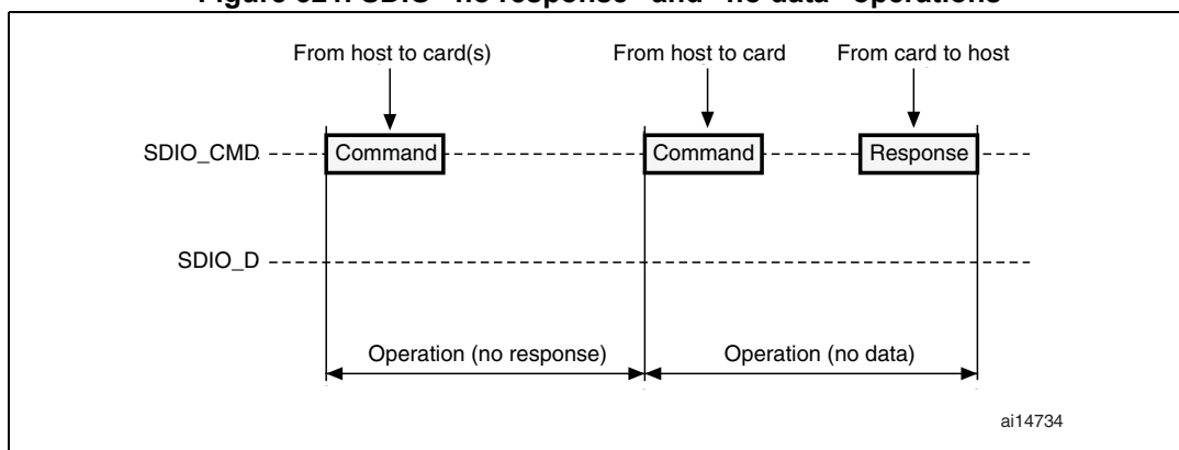
Figure 321. SDIO “no response” and “no data” operations
