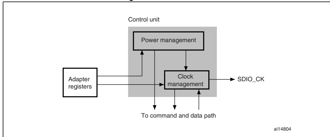
Figure 328. Control unit
