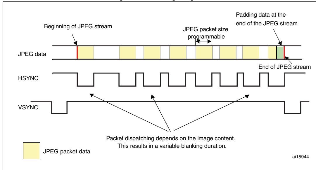
Figure 75. Timing diagram
